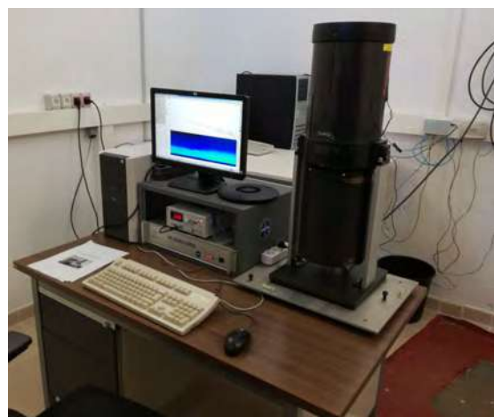
Figure 9.8. The MPL-3 from INTA, at the lidar facility at IZO (installed in October 2018).
