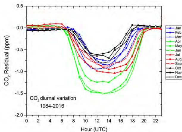
Figure 4.11. Mean diurnal variation of CO 2 residuals for each month of the year in the period 1984-2016. The residuals have been calculated daily as the difference of CO 2 for every hour compared with the night-time (20:00-08:00 UTC) background level.
