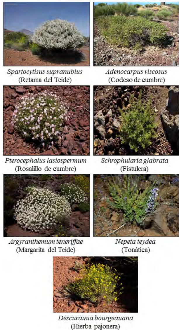
Figure 15.1. Endemic taxa typical from high lands of the island of Tenerife, which are analysed in the Phenology programme.
