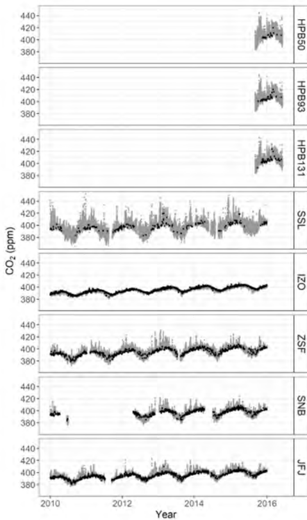
Figure 4.12. Time series plots of validated CO 2 datasets (gray), and selected datasets by ADVS (black) at six GAW stations. Reprinted from Yuan et al. (2018). The comparison indicates that IZO shows the least noisy and most stable CO 2 record of all stations.
