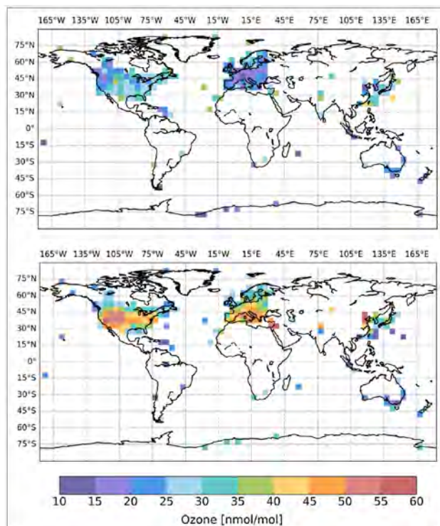
Figure 5.7. Monthly daytime (8–20 h local time) average ozone mole fractions during 2010–2014 gridded onto a 5^\circ \times 5 longitude-latitude grid. Top: January, bottom: July. All stations at altitudes below 2000 m and with at least 3 years of data during the interval were included. (Reprinted from Schultz et al., 2017).
