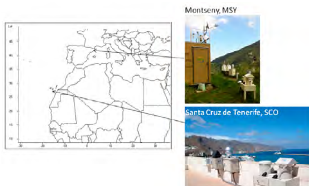
Figure 8.7. Map of the sites used in this study, Montseny (MSY) Santa Cruz de Tenerife (SCO). In the forefront of both instrument photos the wet/dry deposition collectors are shown. Reprinted from Castillo et al. (2017).
