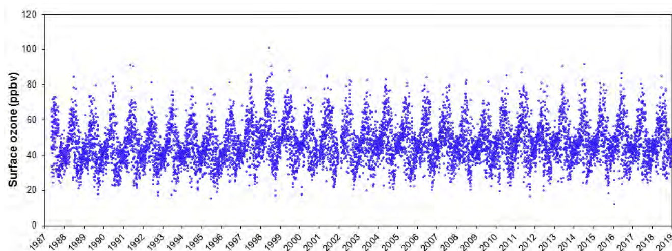
Figure 5.2. Long-term daily (night period) surface O 3 at IZO (1987-2018).
