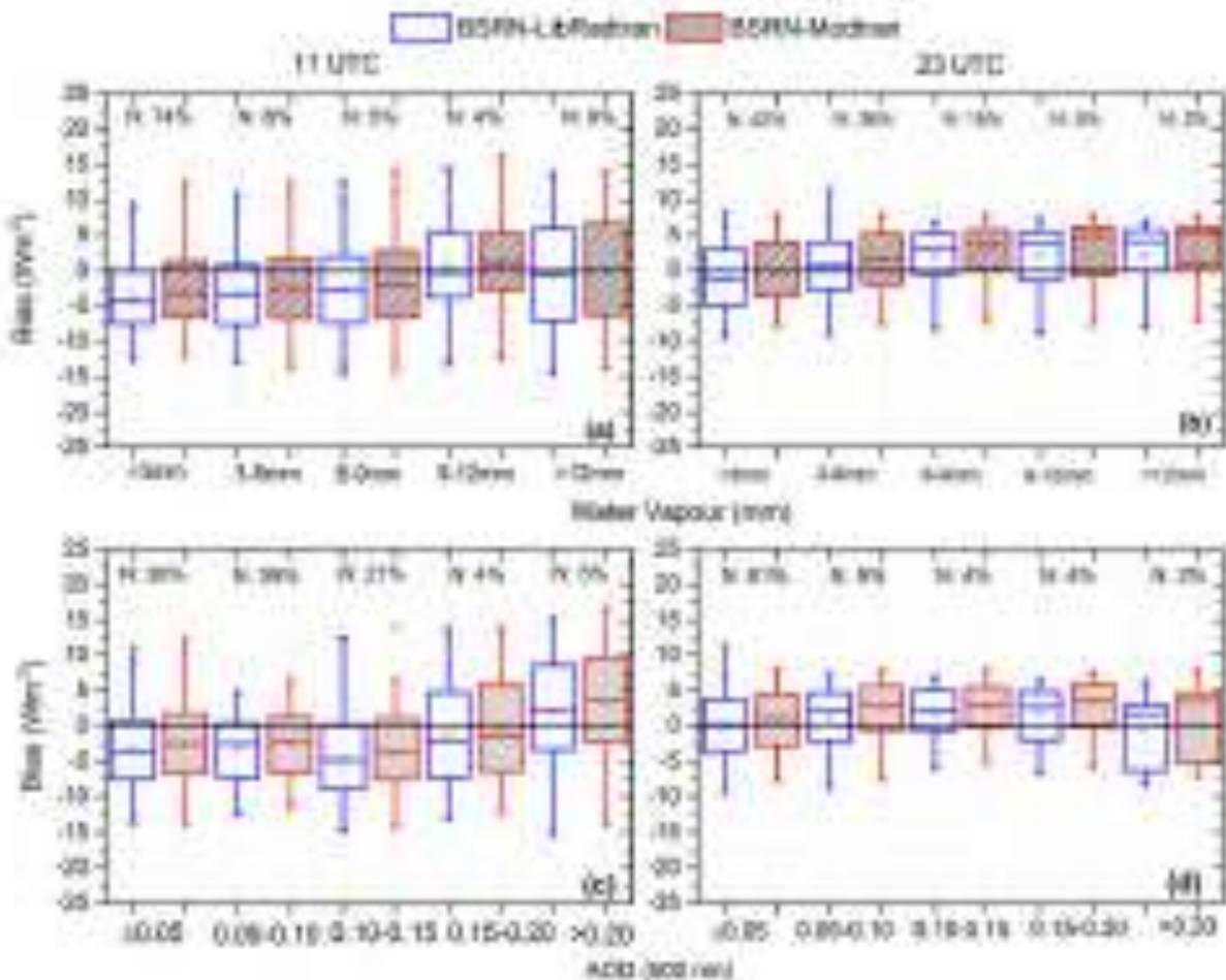
Figure 10.5. Box plot of mean LDR bias (model-BSRN in W m^{-2} ) vs. PWV (mm) (a) at daytime (b) at night-time, and vs. AOD (500 nm) (c) at daytime and (d) at night-time between 2010 and 2016. Lower and upper boundaries for each box are the 25 th and 75 th percentiles; the solid line is the median value; the crosses indicate values out of the 1.5-fold box area (outliers) and hyphens are the maximum and minimum values. The blue boxes represent LibRadtran/BSRN and the red ones represent MODTRAN/BSRN. N indicates the number of measurements in each interval. Shadings show the range of instrumental error ( \pm 3 W m^{-2} ). Reprinted from García et al. (2018).
