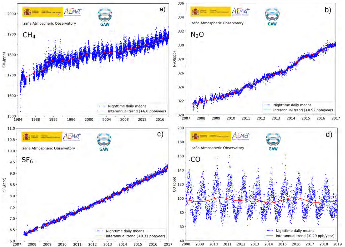
Figure 4.4. Izaña Atmospheric Observatory time series for a) CH 4 , b) N 2 O, c) SF 6 and d) CO.
