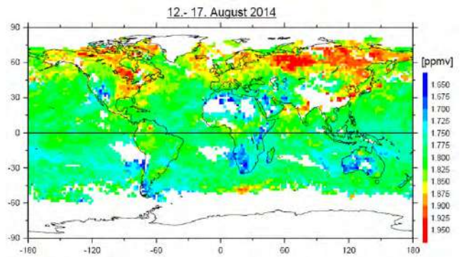
Figure 7.10. MUSICA/INMENSE IASI CH 4 concentrations at 4.2 km altitude for mid-August 2014 averaged for a latitude×longitude area of 2°×2°. Reprinted from García et al., (2018).
