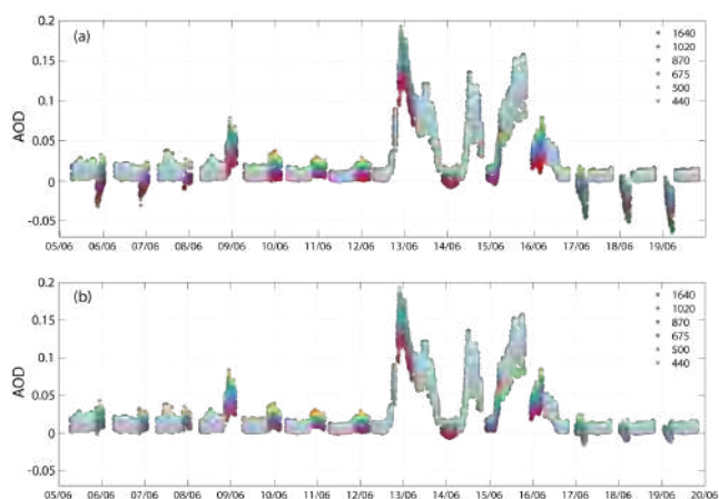
Figure 20.7. AOD evolution for one Moon cycle (June, 2014) at Izaña. Opaque colors represent daylight data. Nocturnal AOD before (a) and after (b) correction is plotted.
