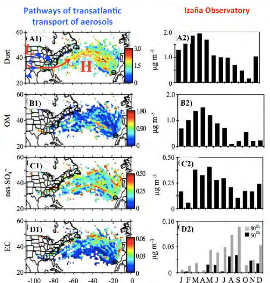
Figure 8.6. Median Concentration At Receptor (MCAR) plots (left column) and monthly value of the 50th percentile (right column) for dust, organic matter (OM), non-sea-salt-sulfate ( \text{nss-SO}_4^- ) and elemental carbon (EC). Reproduced from García et al. (2017b).
