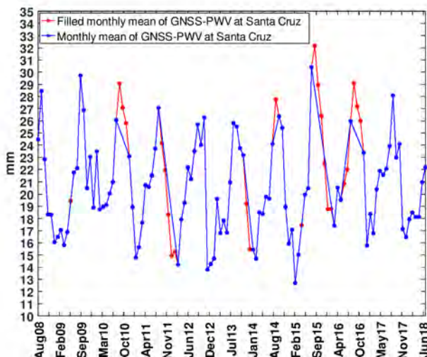
Figure 12.7. PWV monthly data series at SCO (2008-2018).
