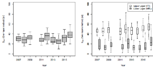
Figure 20.13. Lidar ratio at 523 nm from one-layer (left) and two-layer methods (right) for each year between 2007 and 2017. The central rectangles extend from the first quartile to the third quartile and the median is represented by a horizontal line. The whiskers are defined as the upper and lower quartiles \pm 1.5 IQR (inter-quartile range). Reprinted from Berjón et al. (2019).
