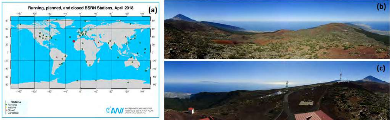
Figure 10.6. (a) Location of the Izaña station (IZA) on a global map of all BSRN stations http://bsrn.awi.de . Views of Izaña radiation station: (b) Northern and Eastern Views (Azimuth 360°, Inclination 0° degrees; Azimuth 90°, Inclination 0° respectively) (c) Southern and Western Views (Azimuth 180°, Inclination 0° and Azimuth 270°, Inclination 0°, respectively). Reprinted from García et al. (2019).
