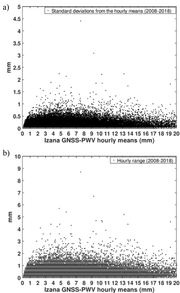
Figure 12.3. a) Dependency of the hourly standard deviation and b) hourly range with respect to the GNSS-PWV hourly mean at IZO during 2008-2018.
