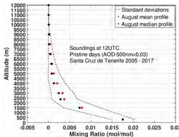
Figure 12.19. August mean and median water vapour vertical profile from Tenerife radiosondes for pristine days only, 2005-2017.
