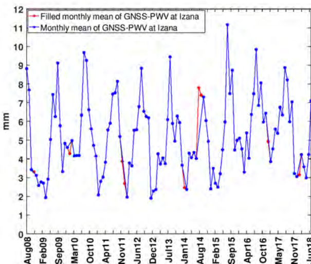
Figure 12.8 PWV monthly data series at IZO (2008-2018).
