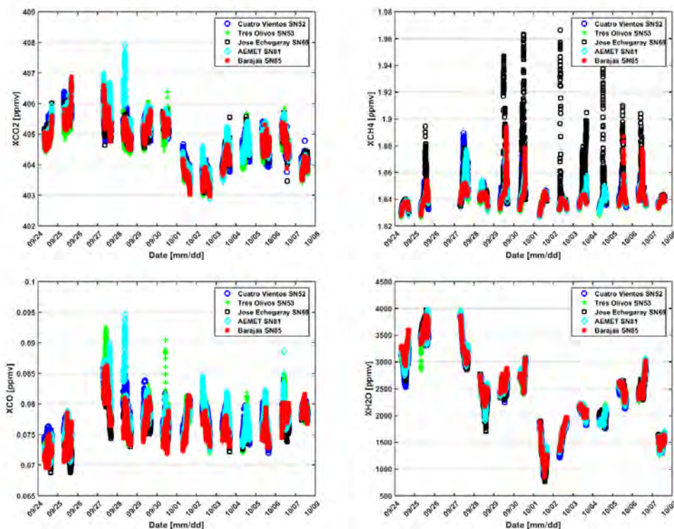
Figure 7.8. Time series of the total column-averaged abundances of carbon dioxide (XCO 2 ), methane (XCH 4 ), carbon monoxide (XCO) and water vapour (XH 2 O) as observed by five COCCON EM27/SUN spectrometers during the scientific campaign MEGEI-MAD in Madrid between 24 th September and 7 th October 2018.
