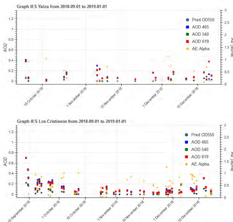
Figure 21.6. Example of measurements available in the web application of the project (Calima Project Graph View). Aerosol optical depth (AOD) at 465 m, 540 nm and 619 nm, Angstrom exponent (alpha) measured at a) IES Yaiza and b) IES Los Cristianos, plotted together with BSC dust forecast at 550 nm (Pred OD550) for 1/9/2018-31/12/2018.
