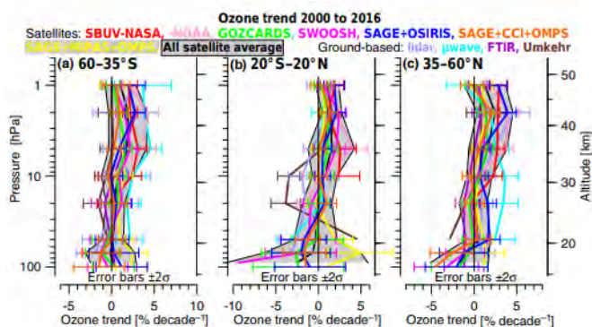
Figure 7.5. Vertical profiles of 2000 to 2016 ozone trends for different merged satellite and ground-based station data sets. Results are for the zonal bands 60 to 35^\circ S (a), 20^\circ S to 20^\circ N (b) and 35 to 60^\circ N (c) (reprinted from Steinbrecht et al., 2017). The HR FTIR data from IZO are included for the 35 to 60^\circ N band.
