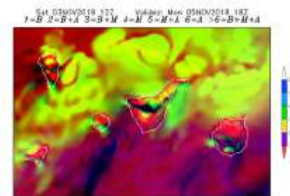
Figure 13.8. Example of graphics presented in MM5 web page. This shows the plot of the total cloud fraction (low+medium+high) shaded in colours on 5 November 2018 at 18 UTC.
