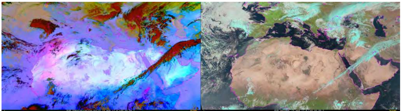
Figure 13.3. Two different RGB composite images from Meteosat-10 satellite for a dust event on 18/04/2017 08:00 UTC. Left panel: dust (channels 7, 9 and 10), right panel: natural (channels 1, 2 and 3).
