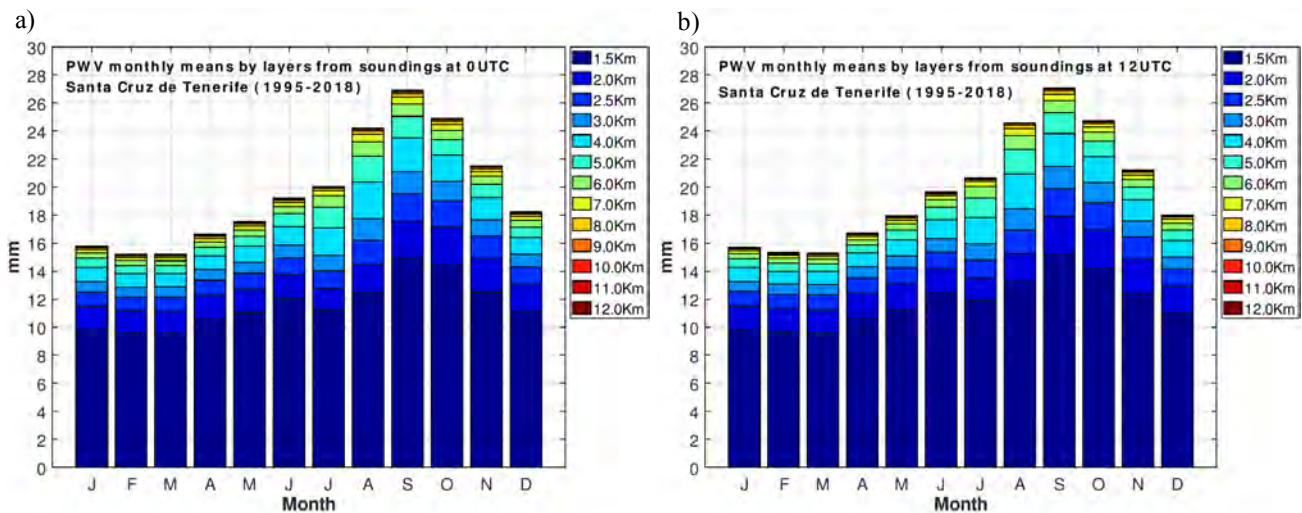
Figure 12.12. Monthly statistics of precipitable water vapour vertical distribution from Tenerife radiosondes: a) 00UTC and b) 12UTC, (1995-2018).
