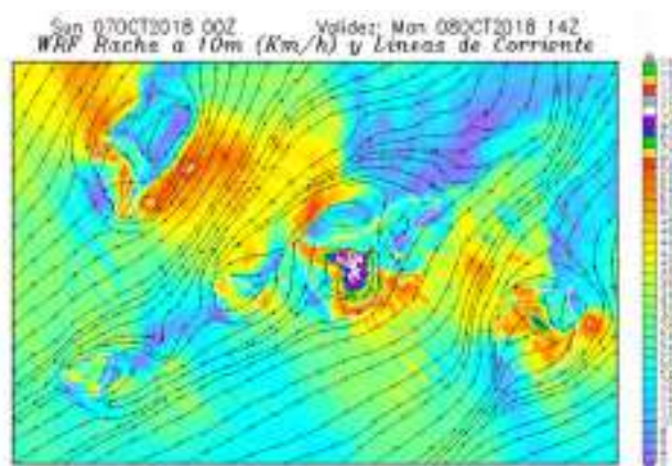
Figure 13.9. Example plot of forecasted wind gust velocity shaded in colours, overlapped with stream lines for a high wind speed episode on 8 October 2018 at 14 UTC.
