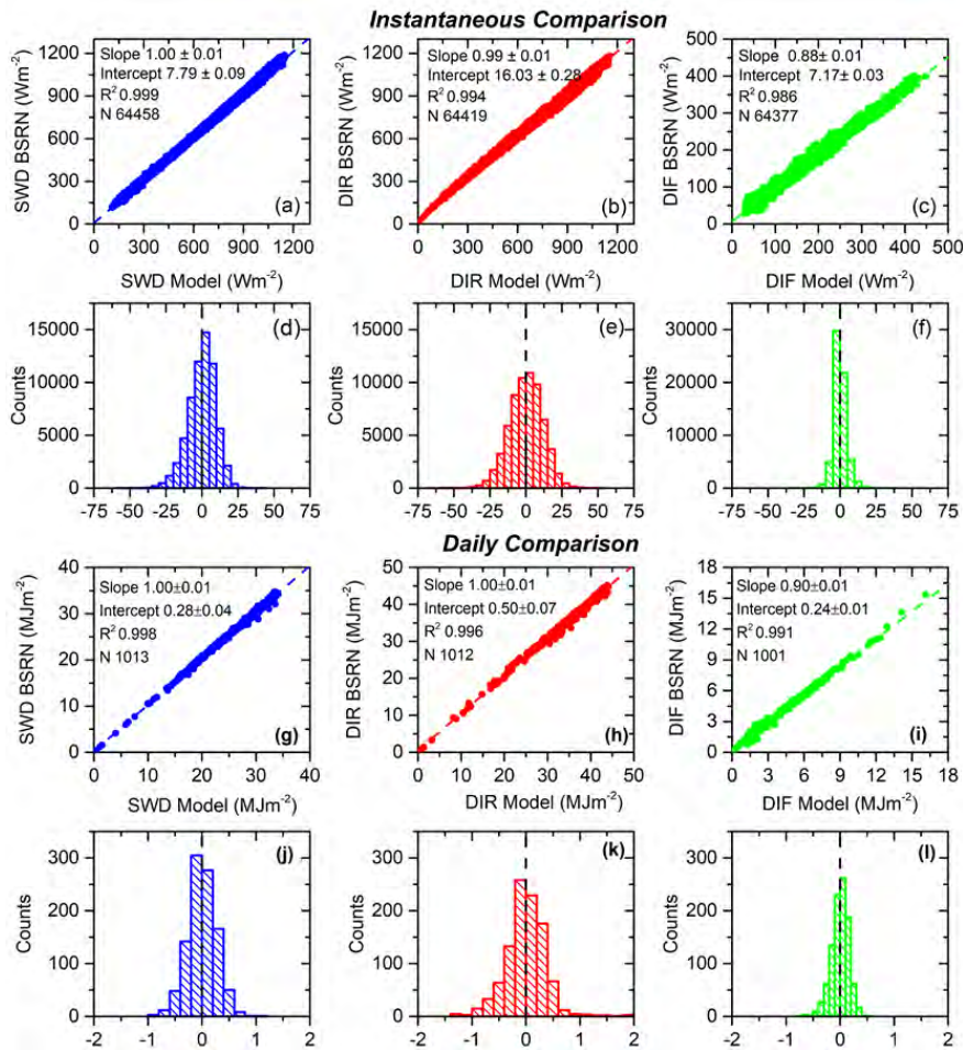
Figure 10.7. Scatterplots and histograms of the instantaneous ( Wm^{-2} ) and daily ( MJ m^{-2} ) radiation measurements and simulations for the period 2009–2017: (a, d, g, j) SWD, (b, e, h, k) DIR and (c, f, i, l) DIF. The fitting parameters are shown in the legend. Reprinted from García et al. (2019).
