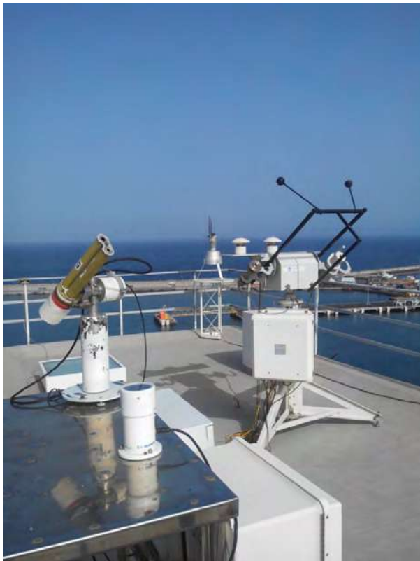
Figure 3.8. Image of Santa Cruz Observatory instrument terrace: ZEN-41-R radiometer (in the foreground), Cimel AERONET photometer, radiation instruments mounted on the sun-tracker and the HIRST pollen sampler (in the background).
