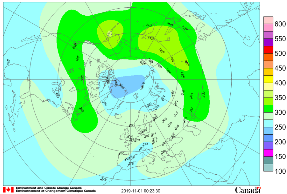
Mean total ozone (DU), 2019/10/01-2019/10/31
