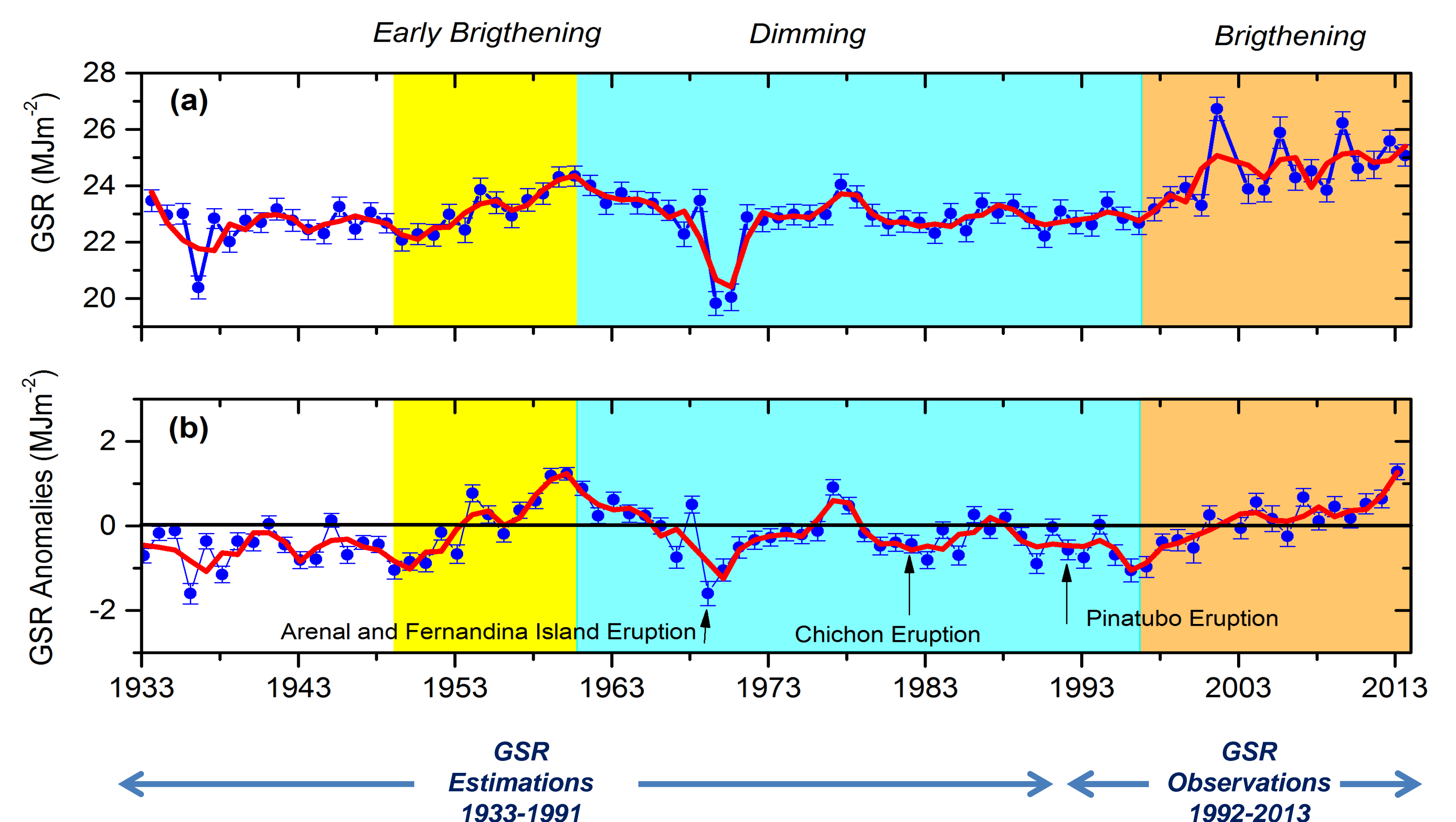
Figure 4.- Time series of the annual means of the (a) GSR and (b) GSR anomalies from 1933 to 2013 at IZA. The error bars indicate \pm 1 SEM (standard error of the mean) The arrows indicate the eruptions of Arenal and Fernandina (1968), Chichón (1982) and Pinatubo (1991). Five-yr moving average is shown in red. Time series has been deseasonalised by subtracting the averaged GSR annual cycle, obtaining the annual mean anomalies time series.
