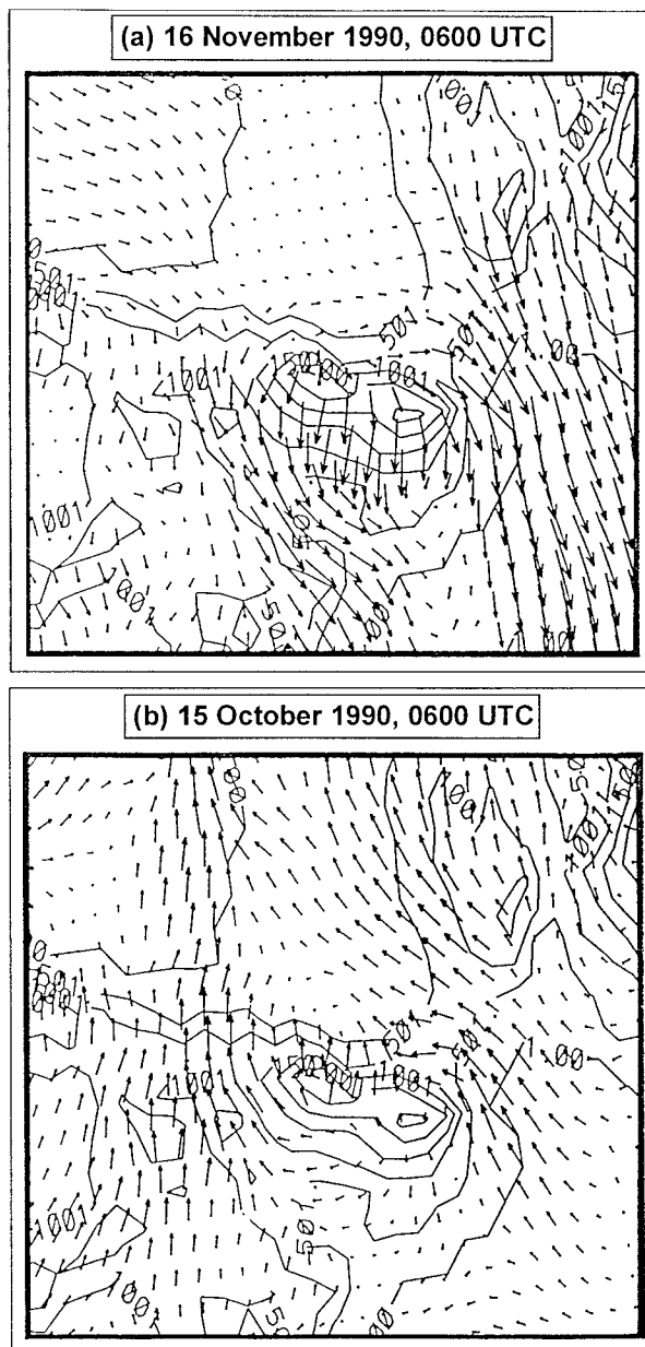
FIG. 8. Analysis of ground-level winds at 0600 UTC for (a) northerly synoptic flow on 16 November 1990 during IOP 9 and (b) southerly synoptic flow on 15 October 1990 during IOP 3 over a topographic map of the Pyrénées area.
