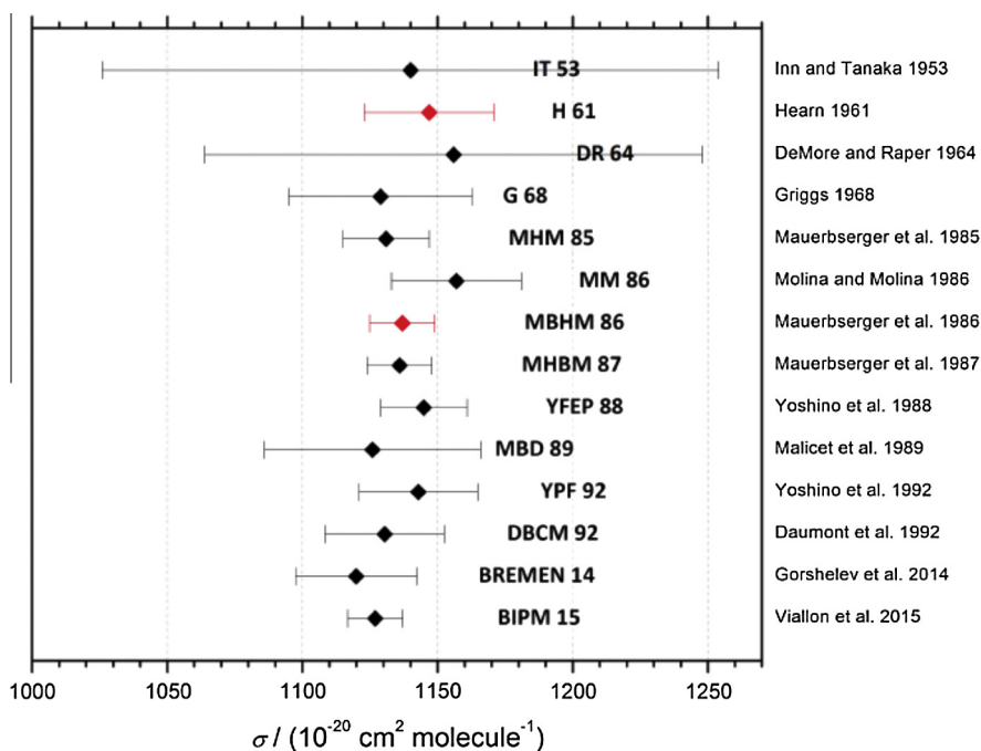
Fig. 4. Summary of laboratory measurements in the Hartley band at 253.65 nm (BIPM). Note the dispersion of the different measurements and the values that are currently used as reference values by different communities (red diamonds). (For interpretation of the references to colour in this figure legend, the reader is referred to the web version of this article.)
