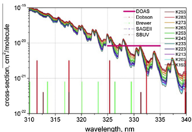
Fig. 3. New measurements of ozone absorption cross-sections at different temperatures (193–293 K) temperature in the Huggins bands [7,8] including wavelengths indicated as used for different instruments.
