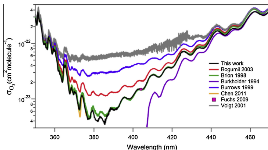
Fig. 2. Measurements of ozone absorption cross-sections at room temperature in the absorption minimum between the Huggins and Chappuis bands [38]. Note the very good agreement with the previous measurements of Brion et al. [4].
