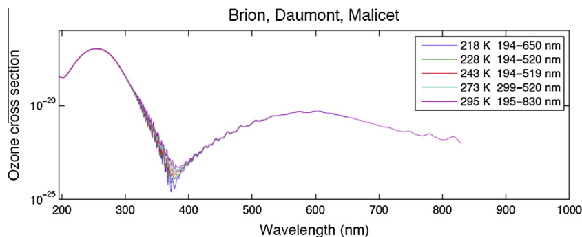
Fig. 6. Brion-Daumont-Malicot (BDM) cross-sections.
