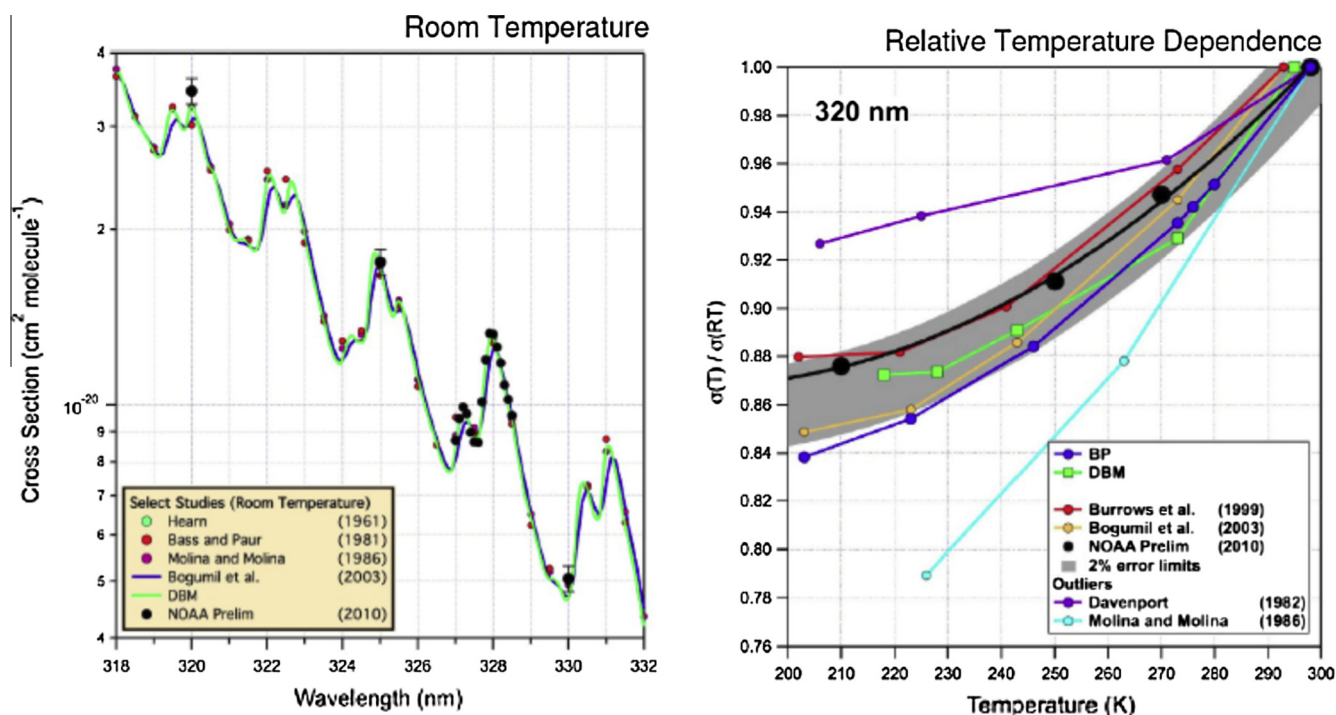
Fig. 1. Measurements of ozone absorption cross-sections and their temperature dependence in the Huggins bands (Burkholder et al. unpublished). Note the good agreement with previous measurements of Burrows et al. [43] and BDM (1998).
