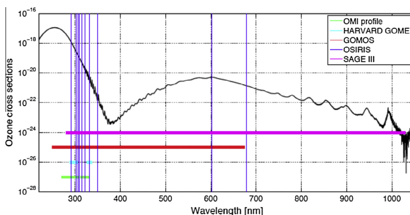
Fig. 10. Ozone cross-sections at one temperature (black line) and examples of wavelength regions used for instruments/algorithms providing ozone profiles.
