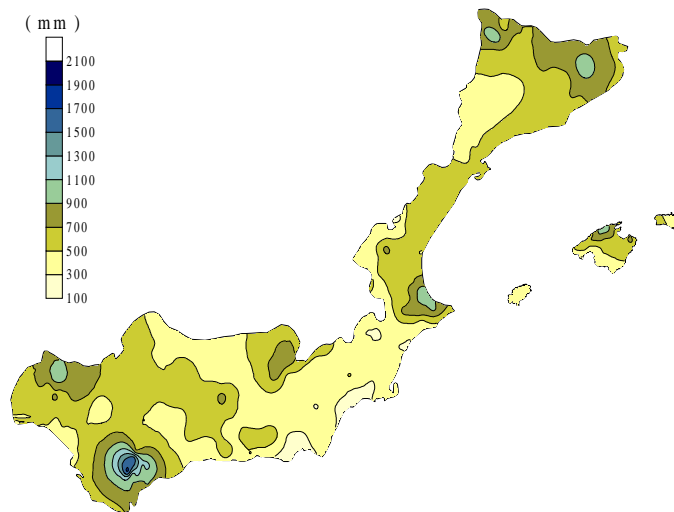
Fig 2. Yearly mean precipitation for 1984-93
