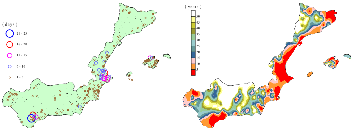
Fig 3. Days with extreme rainfalls (> 100 mm) during 1984-93 (left). Recurrence intervals of 100 mm events, for 1984-93 (right)
