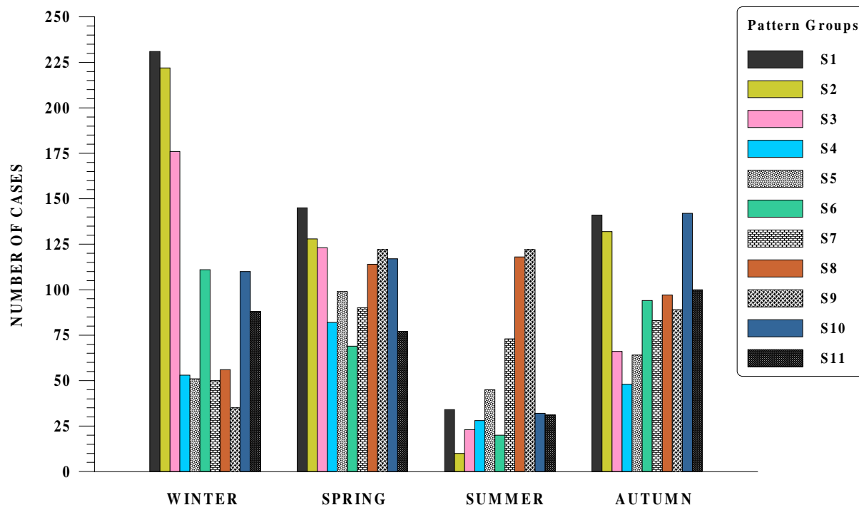
Fig 5. Seasonal distribution for the 11 pattern groups of significant daily rainfall
