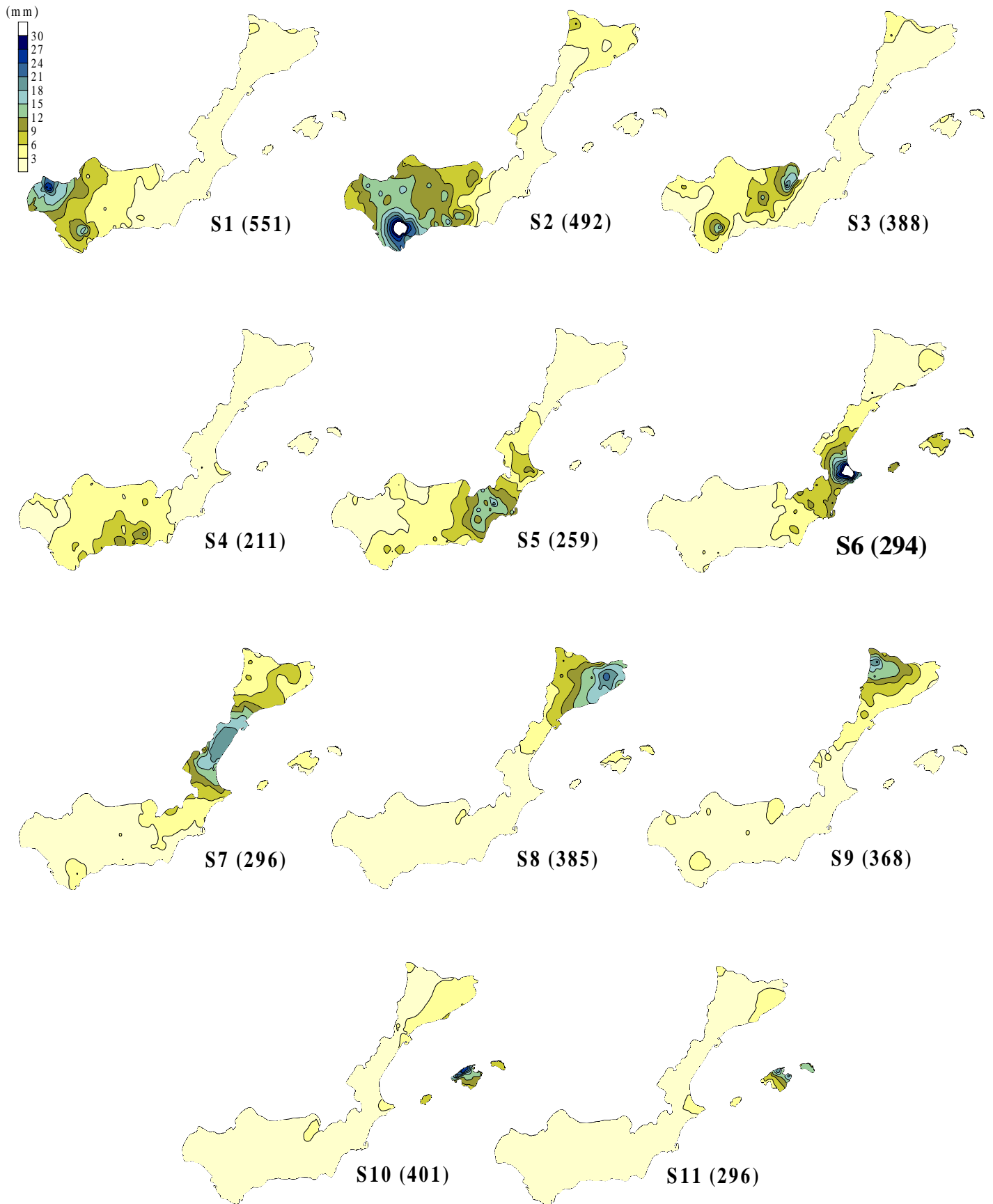
Fig 4. Daily rainfall composites for the 11 pattern groups of significant rainfall in Mediterranean Spain. The number of days for 1964-93 included in each pattern group is indicated in parentheses (total, 3941)
