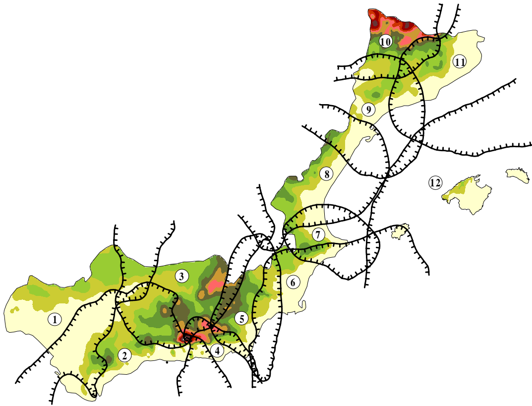
Fig 6. Daily rainfall affinity areas in Mediterranean Spain, resulting from an overlapping regionalization (threshold loading for the regions is 0.25)
