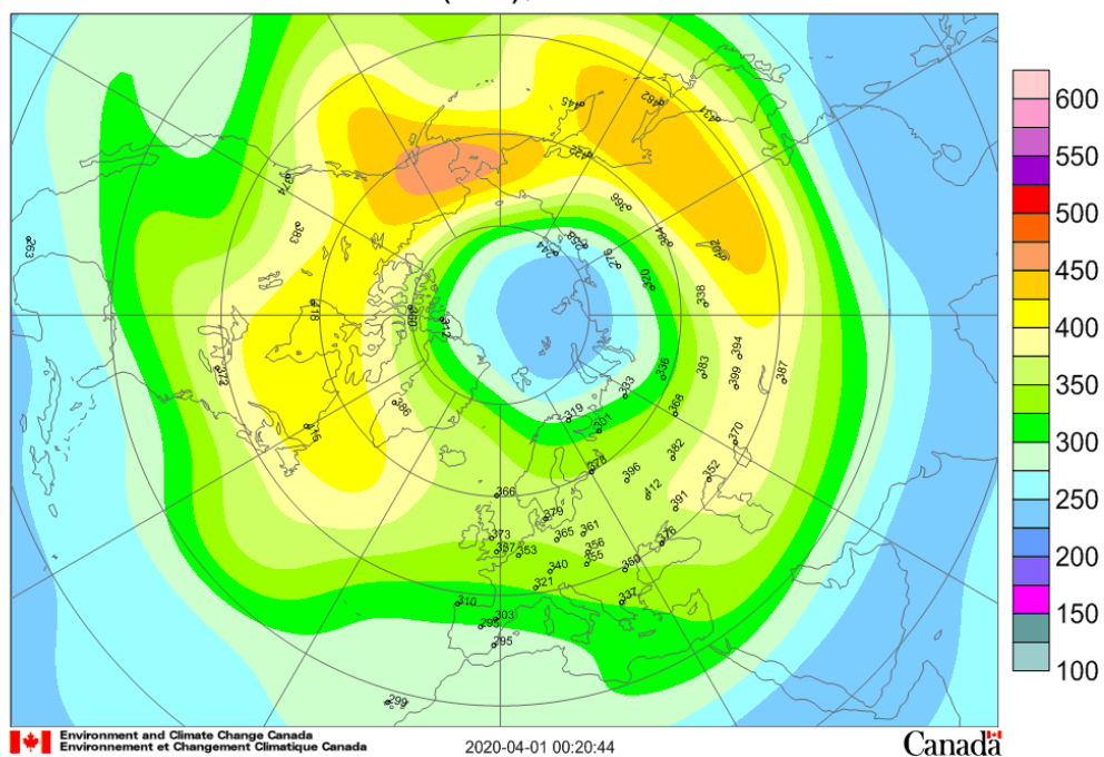
Mean total ozone (DU), 2020/02/01-2020/02/29
