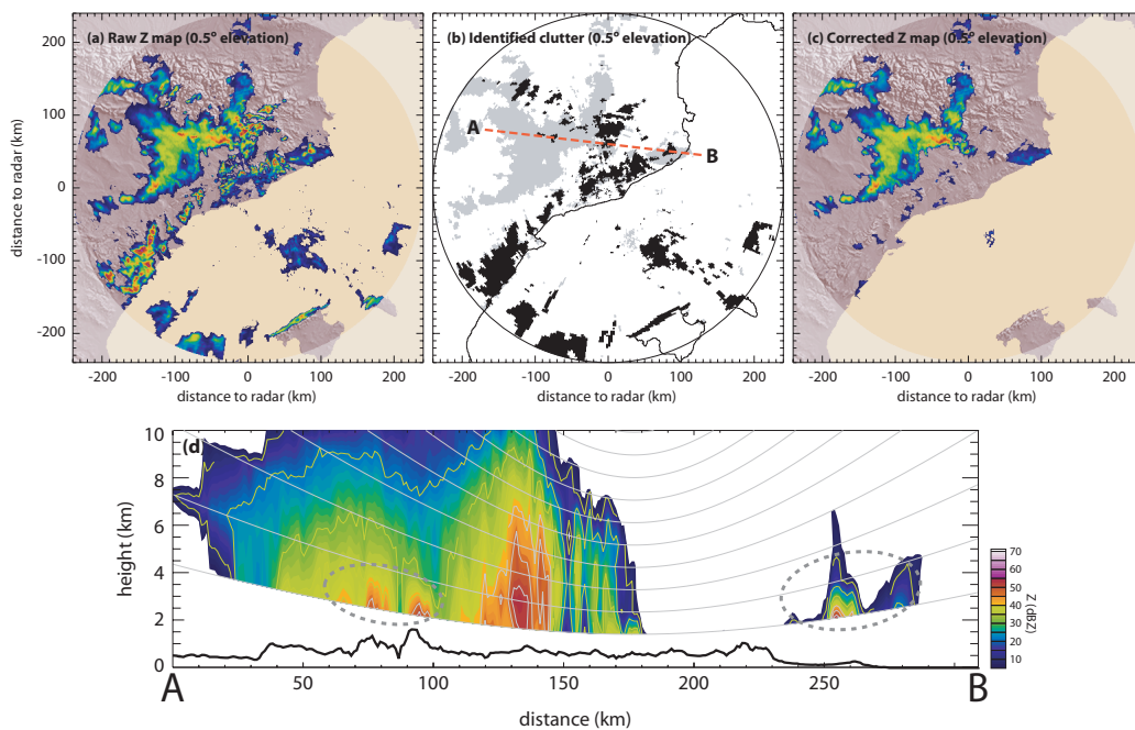
Fig. 9. Same as Fig. 6 but for the radar scan measured on 14 August 2001 at 1010 UTC.
