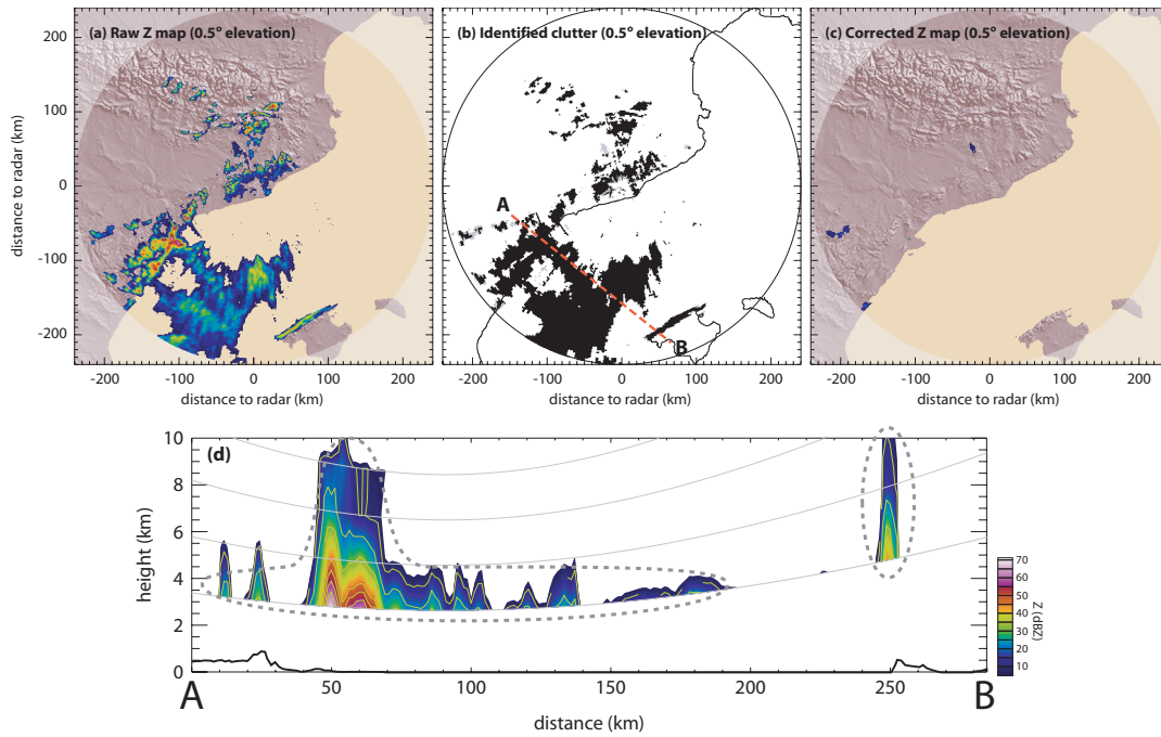
Fig. 6. Identification of non-meteorological echoes in the radar scan measured on 17 July 2001 2000 UTC. (a) Raw reflectivity map corresponding to the first tilt ( 0.5^\circ elevation). (b) In black, bins identified as clutter in the raw reflectivity field (areas where Z > 5 dBZ are depicted in grey). (c) Corrected reflectivity field (after removing clutter bins and filling the resulting gaps). (d) Vertical cross section interpolated from raw volumetric radar measurements along the line A-B of (b). Dashed line encircles most relevant clutter echoes. Beam paths have been calculated assuming Normal Propagation conditions.
