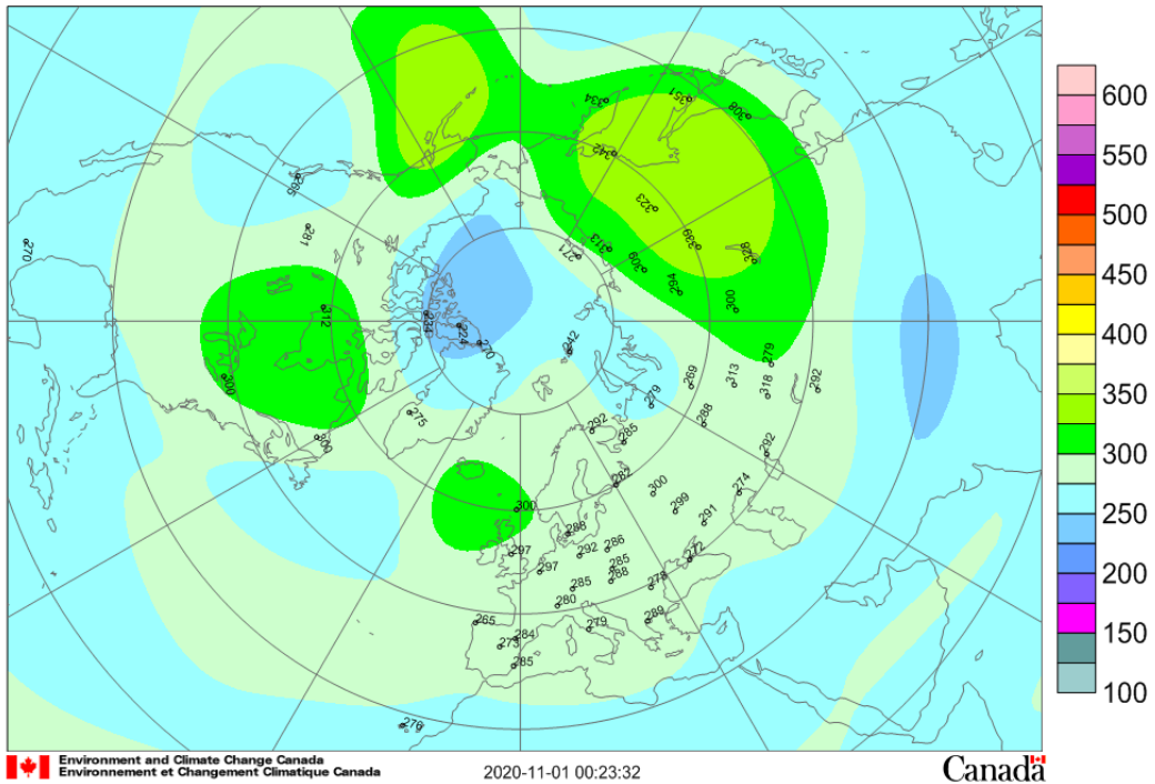
Mean total ozone (DU), 2020/10/01-2020/10/31
