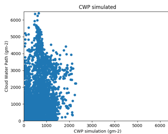
Figure 38. CWP scatter plot the 14th September 2019 at 14:00Z over Spain
