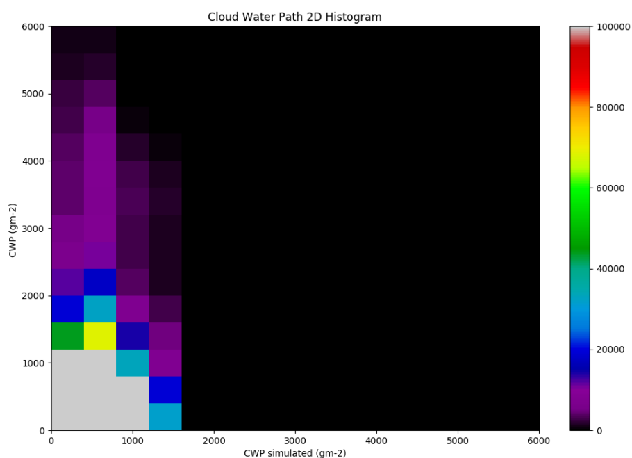
Figure 40 Cloud Water Path two dimensions histogram evaluated for Spain from May to September between 10:00Z and 15:00Z every thirty minutes
