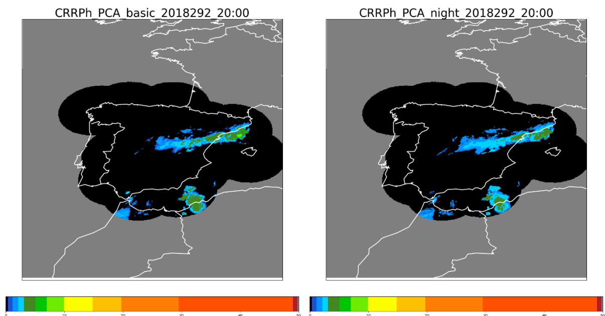
Figure 26. CRRPh night algorithm instantaneous rain rate intensities ( \text{mmh}^{-1} ) basic output, over Spain the 19 th October 2018 at 20:00Z with 9 inputs, including the pseudo-VIS06 and pseudo-CWP on the left. CRRPh night algorithm with 7 inputs, not including the additional pseudo-variables on the right.
