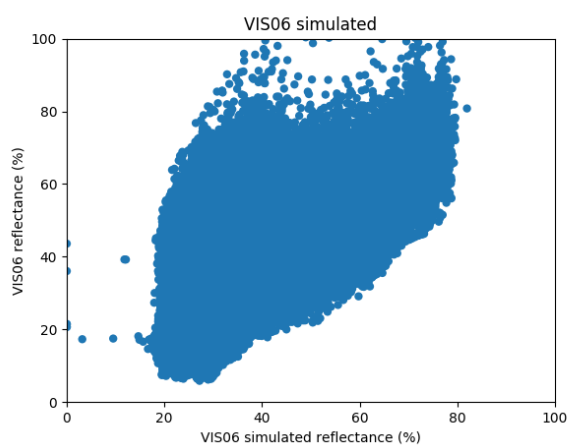
Figure 37. VIS06 scatter plot the 13th September 2019 at 14:30Z over Spain
