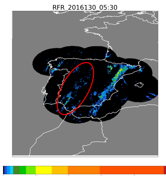
Figure 28. Spanish composite radar ( \text{mmh}^{-1} ) over Spain the 9 th May 2016 at 05:30Z
