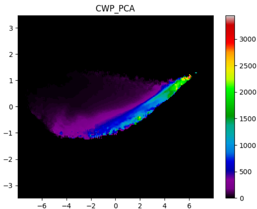
Figure 34. 200*200 LUT for CWP
