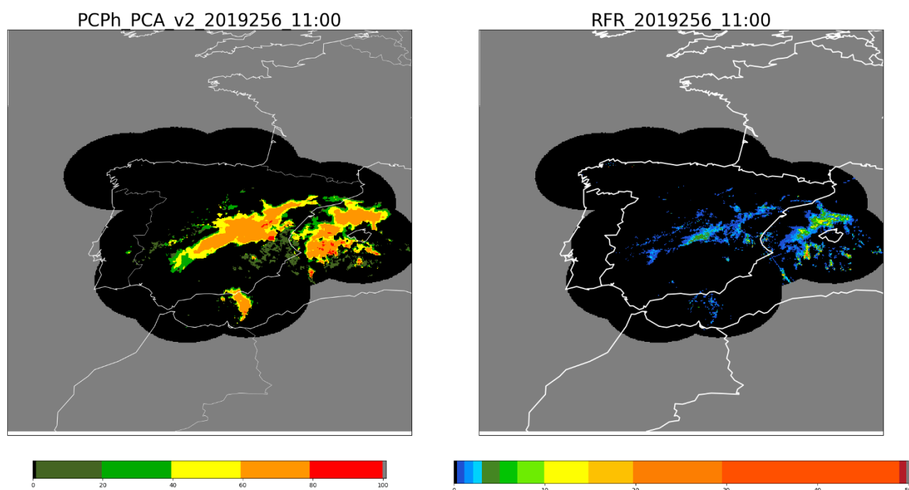
Figure 30. PCPh Probability of precipitation (%) over Spain the 13 th September 2019 at 11:00Z on the left side. Spanish composite radar (mmh -1 ) on the right side.
