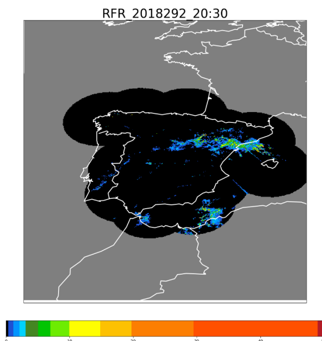
Figure 25. Spanish composite radar ( \text{mmh}^{-1} ) over Spain the 19 th October 2018 at 20:30Z
