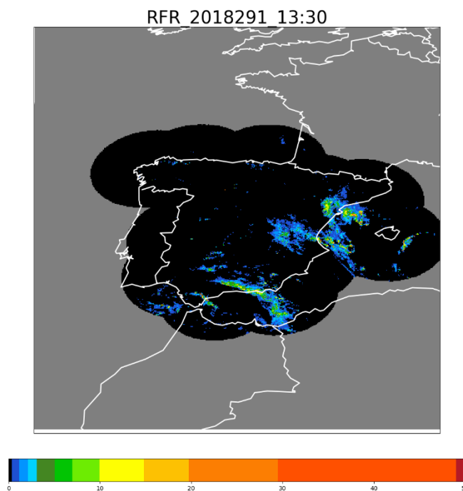
Figure 23. Spanish composite radar ( \text{mmh}^{-1} ) over Spain the 18 th October 2018 at 13:30Z
