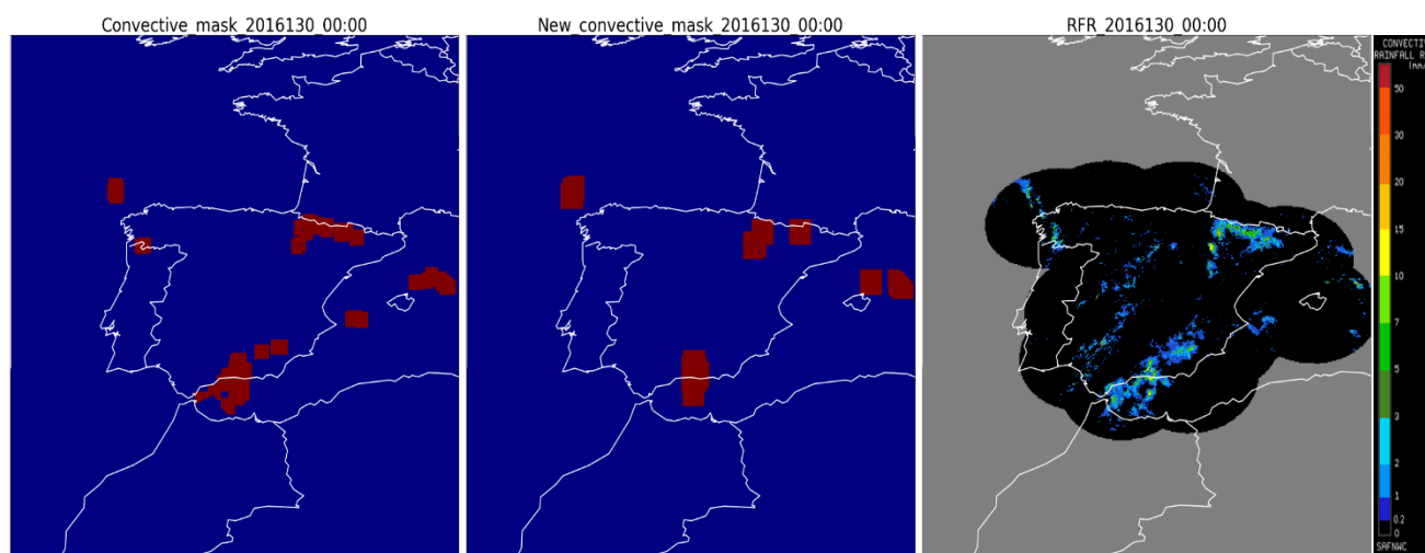
Figure 18. Calibrating convective box areas, for previous CRRPh version(left),and for the current CRRPh (middle).Spanish composite radar on the right side.
