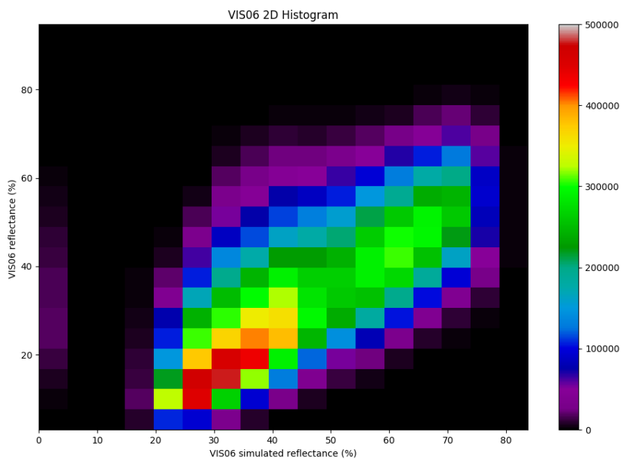
Figure 39. VIS06 two dimensions histogram evaluated for Spain from May to September between 10:00Z and 15:00Z every thirty minutes
