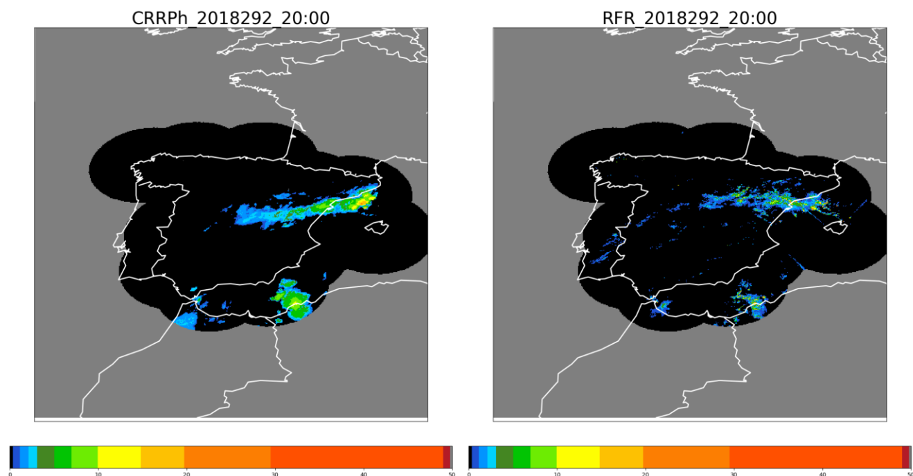
Figure 21 CRRPh instantaneous rain rate intensities ( \text{mmh}^{-1} ) over Spain the 19 th October 2018 at 20:00Z on the left side. Spanish composite radar ( \text{mmh}^{-1} ) on the right side.
