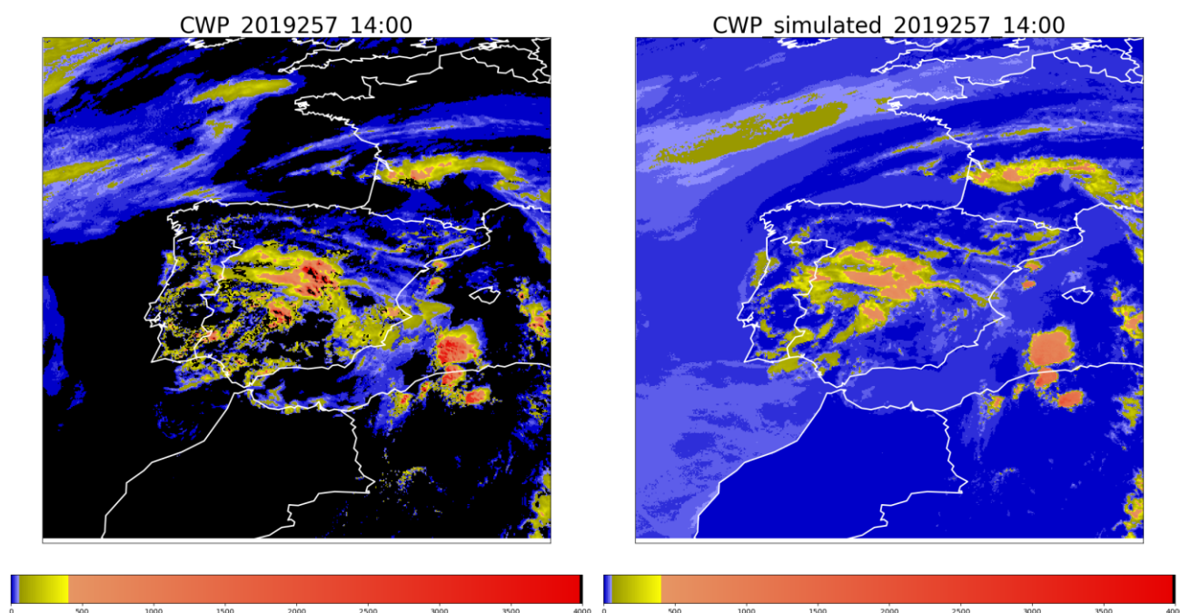
Figure 36 Cloud Water Path ( \text{gm}^{-2} ) simulation over Spain the 14th September 2019 at 14:00Z
