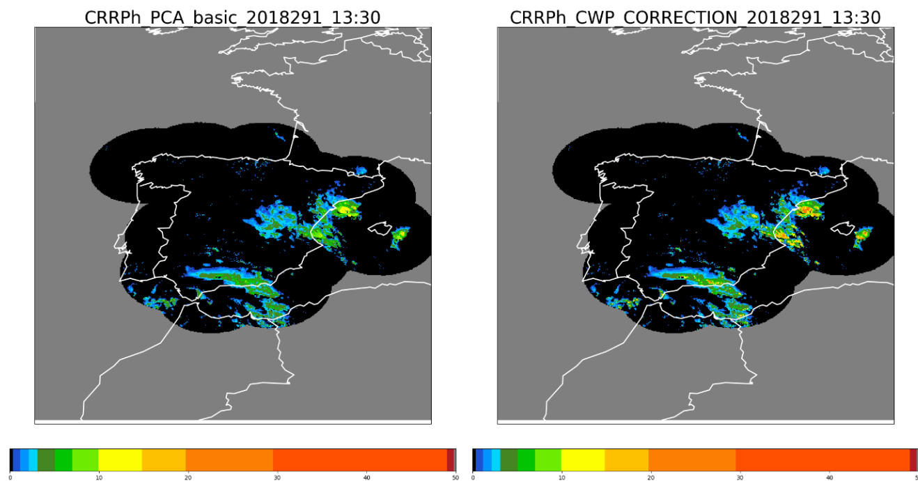
Figure 22 CRRPh instantaneous rain rate intensities ( \text{mmh}^{-1} ) over Spain the 18 th October 2018 at 13:30Z. Basic output on the left and having applied the CWP correction factor on the right.
