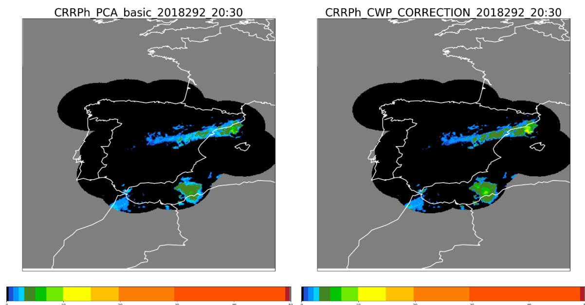
Figure 24. CRRPh instantaneous rain rate intensities ( \text{mmh}^{-1} ) over Spain the 19 th October 2018 at 20:30Z. Basic output on the left and having applied the CWP correction factor on the right.
