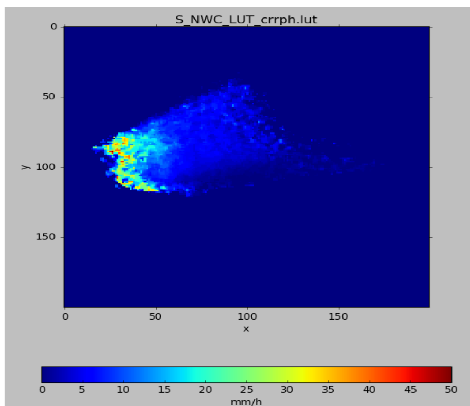
Figure 19. 200*200 calibration LUT for CRRPh
