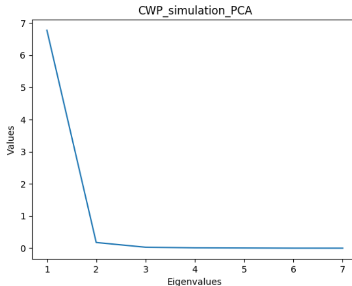
Figure 32. Eigenvalues for CWP and VIS 0.6
