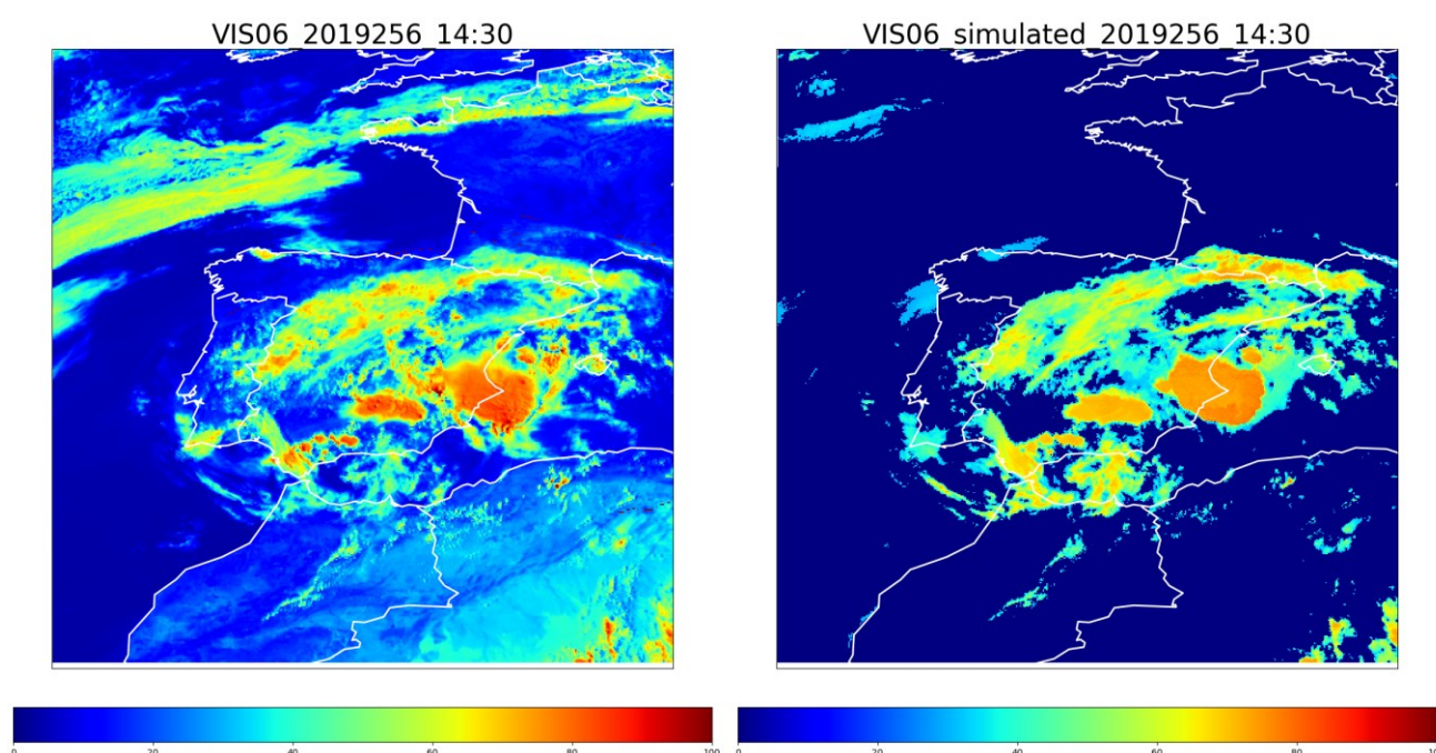
Figure 35. \text{VIS}_{0.6} simulation over Spain the 13th September 2019 at 14:30Z
