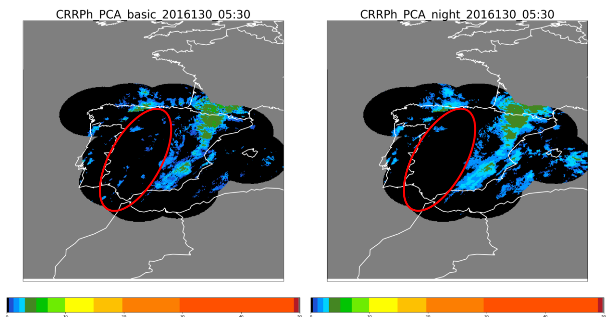
Figure 27. CRRPh night algorithm, instantaneous rain rate intensities ( \text{mmh}^{-1} ) basic output, over Spain the 9 th May 2016 at 05:30Z with 9 inputs, including the pseudo-VIS06 and pseudo-CWP on the left. CRRPh night algorithm with 7 inputs, not including the additional pseudo-variables on the right.
