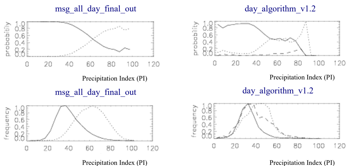
Figure 2 : left: day algorithm tuned on synop collocation data set (dotted: all precipitation). Right: same algorithm, but applied on rain gauge collocation data set (dotted light to moderate precipitation, dashed heavy precipitation). X-axis: Precipitation Index PI
