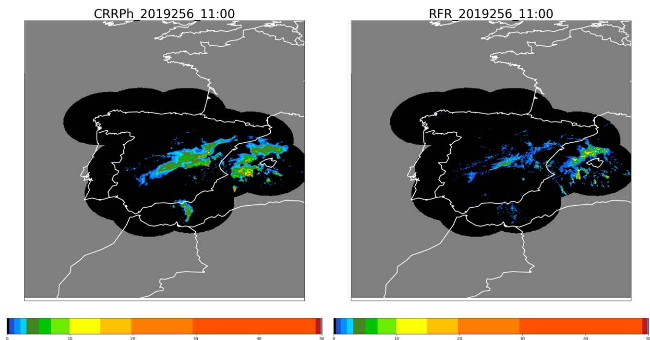
Figure 20. CRRPh instantaneous rain rate intensities ( \text{mmh}^{-1} ) over Spain the 13 th September 2019 at 11:00Z on the left side. Spanish composite radar ( \text{mmh}^{-1} ) on the right side.
