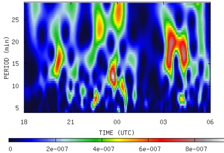
Fig. 9. – Energy of the time series of surface pressure recorded by one of the microbarographs of the array. The wave activity between 2100 and 0500 GMT is clearly visible, with periods between 5 and 30 minutes.
