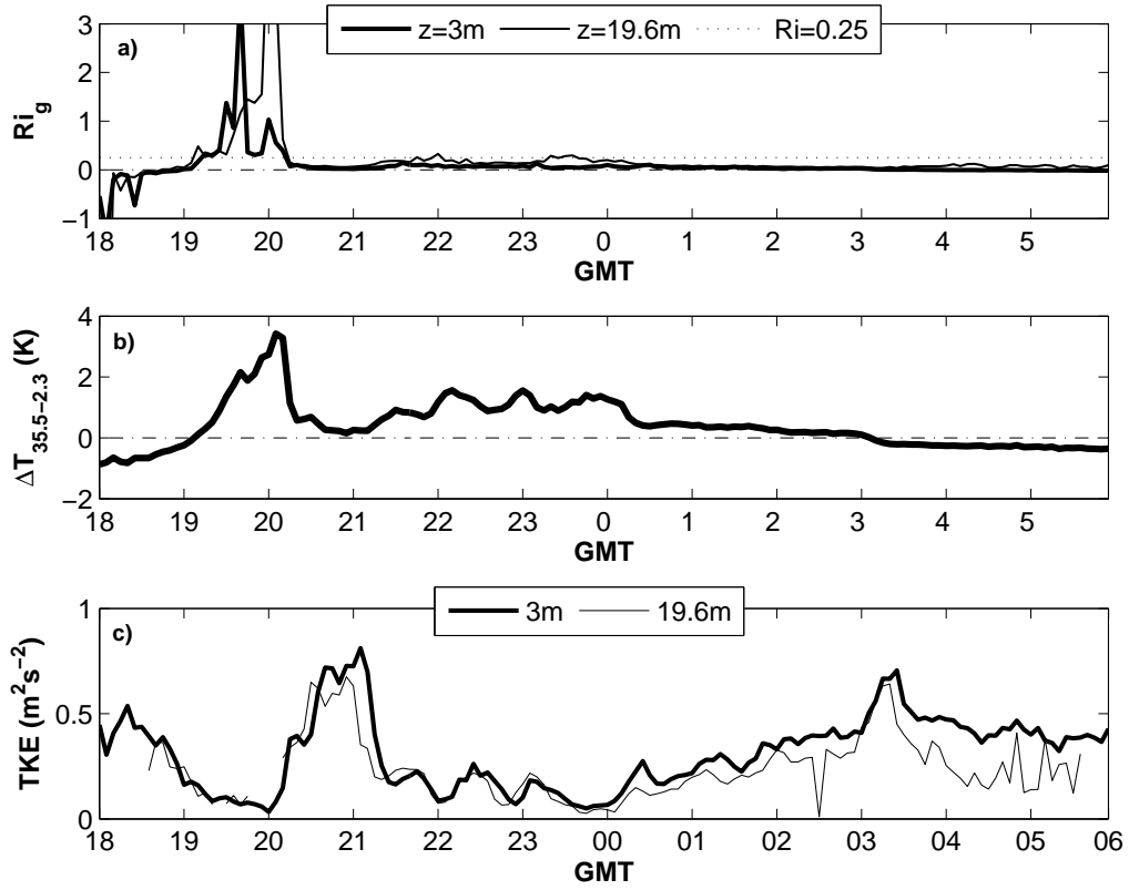
Fig. 4. – Evolution of: a) Gradient Richardson number at 3 and 19.6 m AGL, b) Inversion strength between 35.5 and 2.3 m AGL and c) Turbulent kinetic energy at 3 and 19.6 m. AGL.
