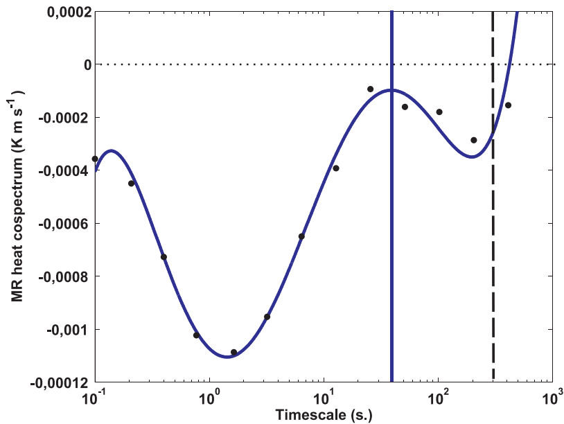
Fig. 1. – Example of a typical MRFD heat cospectrum under stable stratification, and the polynomial fit used to define the gap. Solid and dotted vertical lines mark the timescale of the found gap and the typical 5-min averaging length from the eddy covariance method.
