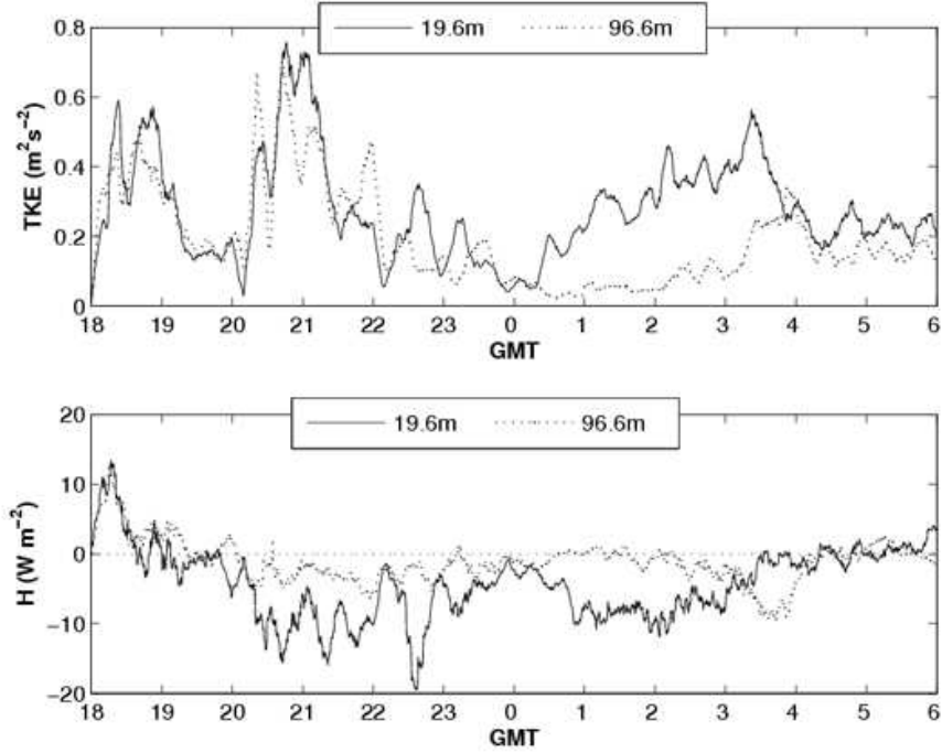
Fig. 13. – a) Turbulent Kinetic Energy and b) vertical heat flux at 19.6 and 96.6 m AGL estimated by means of the wavelet transform.
