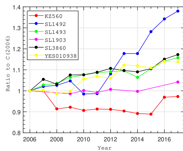
Figure 9. Calibration factor changes of 6 selected broadband filter radiometers.
