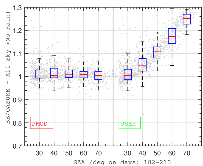
Figure 4. Erythmal weighted broadband irradiance vs. QASUMEII reference data - plotted against the solar zenith angle. Left: WCCUV-calibration (PMOD); right: USER-calibration based on a single calibration factor only. In this example the data of UVE channel of the Kipp & Zonen, SN. 120023, was used. On each box, the central mark indicates the median, and the bottom and top edges of the box indicate the 25 th and 75 th percentiles, respectively. The whiskers extend to the most extreme data points not considering outliers. Outliers are defined as data points outside the 99.3 % confidence interval, assuming a normal probability distribution (MathWorks 2020).
