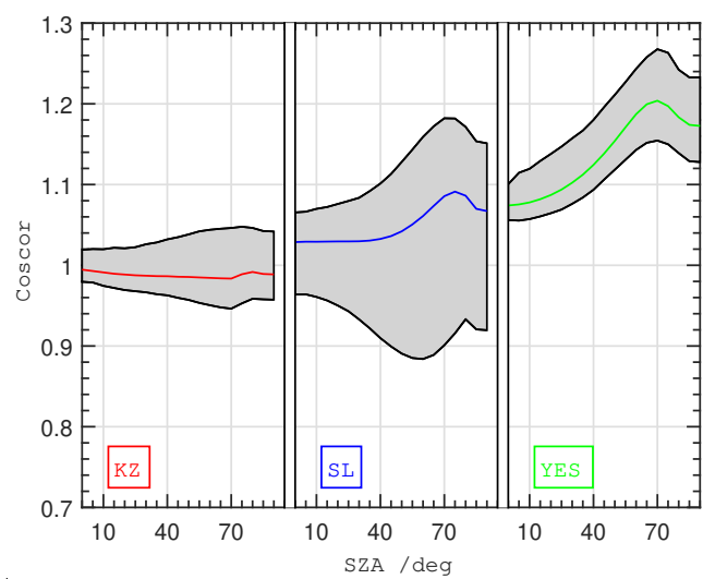
Figure 7. Mean of the cosine correction of the radiometers participating at the UVC-II for a KZ (left), SL (middle) and YES (right) radiometer. The shaded area shows the range of the correction function for the three radiometer types.
