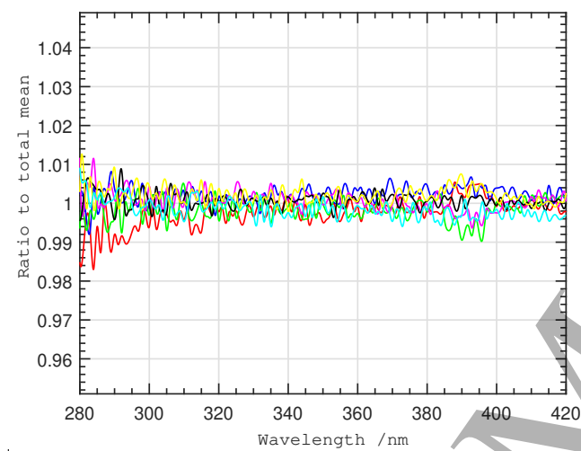
Figure 2. QASUMEII spectral responsivity ratio to the average. The calibrations were based on transfer standard T68523, Day of Year (DOY) 166 till 247, 2017.
