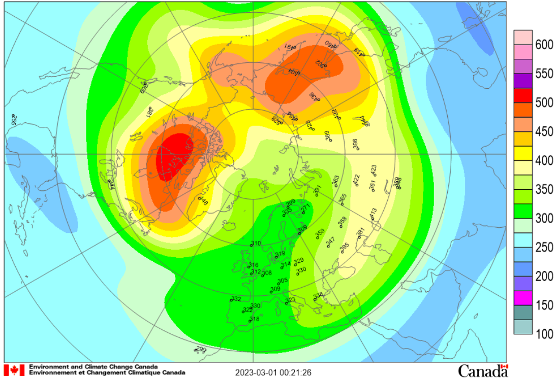
Mean total ozone (DU), 2023/02/01-2023/02/28
