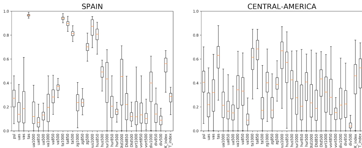
Fig S1: Same as Fig.3 from the main text, but for minimum temperature.
