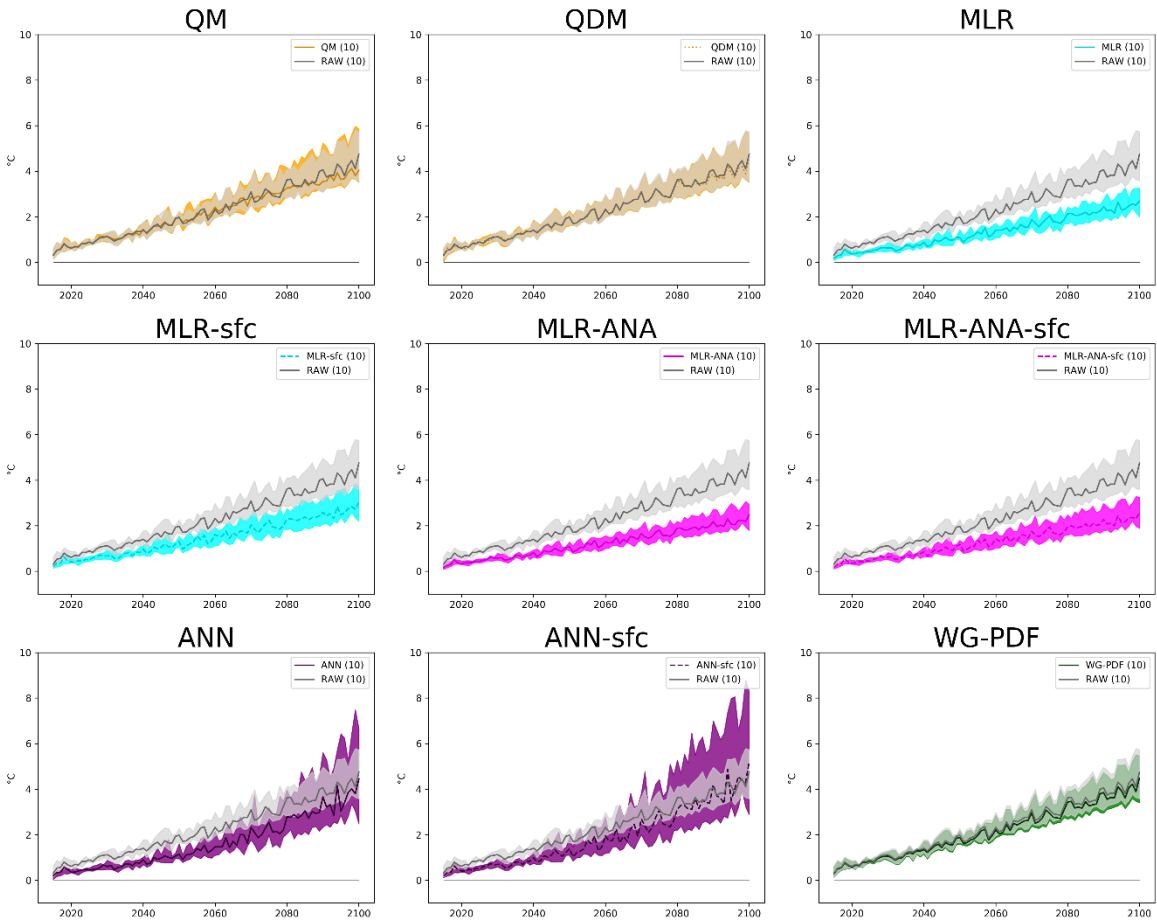
Fig S3: Same as Fig.9 from the main text, but for minimum temperature.
