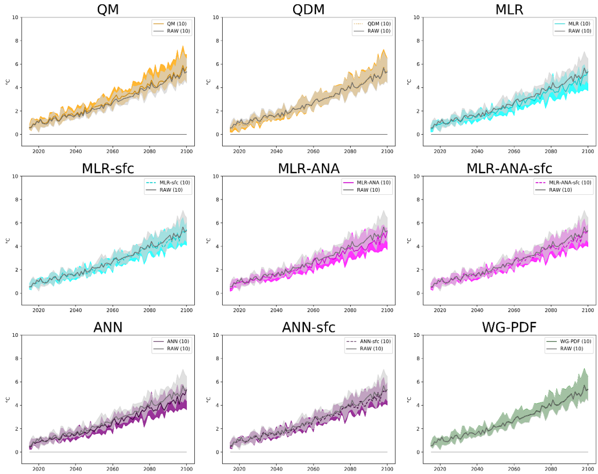
Fig S4: Same as Fig.10 from the main text, but for minimum temperature
