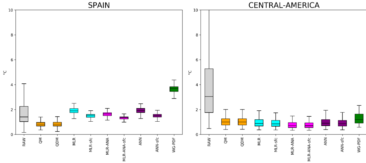
Fig S2: Same as Fig.5 from the main text, but for minimum temperature.
