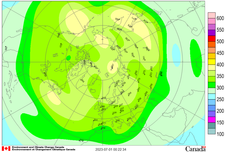
Mean total ozone (DU), 2023/06/01-2023/06/30
