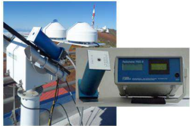
Figure 10.9. Absolute cavity radiometer (PMO6) installed at IZO during summers 2021 and 2022 on the BSRN sun-tracker.
