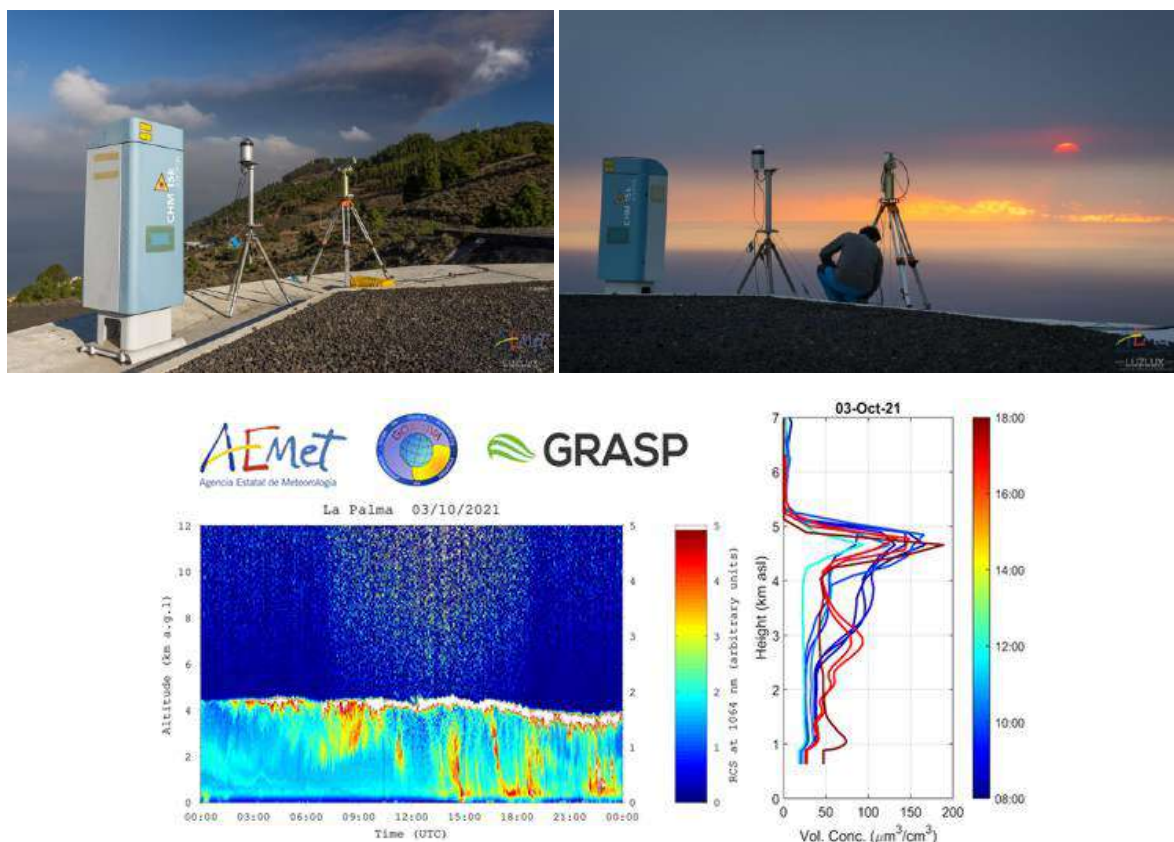
Figure 23.8. Upper panel: Images of instrumentation installed at Fuencaliente station, from left to right: 1) Lufft CHM15k ceilometer, 2) all-sky camera and 3) sun/moon photometer belonging to AERONET. (Image credit: LuzLux). Lower panel: Range Corrected Lidar signal profile extracted from the ceilometer Lufft CHM15k and the corresponding aerosol volume concentration ( \mu\text{m}^3/\text{cm}^3 ) profiles calculated with the GRASP inversion code on 3 October 2021. Reprinted from ACTRIS, 2021.
