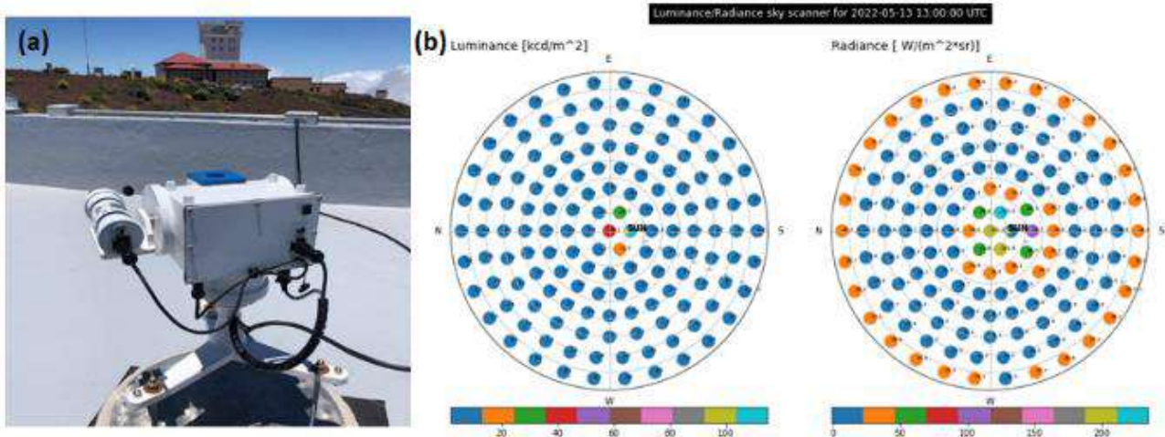
Figure 10.5. (a) The sky scanner EKO MS 321-LR installed at IZO and (b) an example of sky luminance and radiance distribution measurements performed at IZO on 13 May 2022 at 13:00 UTC.
