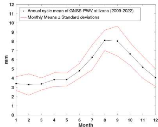
Figure 12.10. GNSS PWV mean seasonal cycle, IZO (2009-2022).
