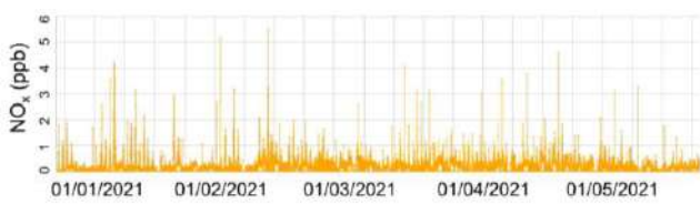
Figure 5.7. 10-minute average of NO x mole fraction (ppb, preliminary data) from January to May 2021 at IZO.
