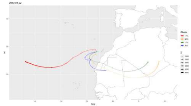
Figure 13.27. Plot representing the mean of the four back-trajectory groups corresponding to 22 January 2010. The legend identifies the percentage of elements in each cluster, and the transparency of the lines indicates the altitude at which they are transported.
