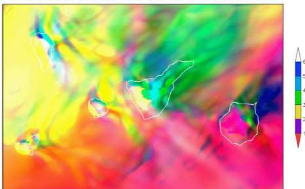
Figure 13.8. Example of graphical representation of total cloud fraction (low+medium+high) shaded in colours on 7 December 2022 at 06 UTC (output of MM5 model).
