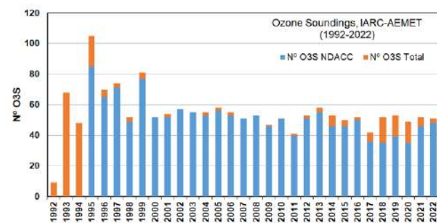
Figure 5.11. Number of ozone soundings (O3S) since the beginning of the programme and the number of ozonesonde datasets recorded in the NDACC database that meet the quality assurance criteria (1992–2022).
