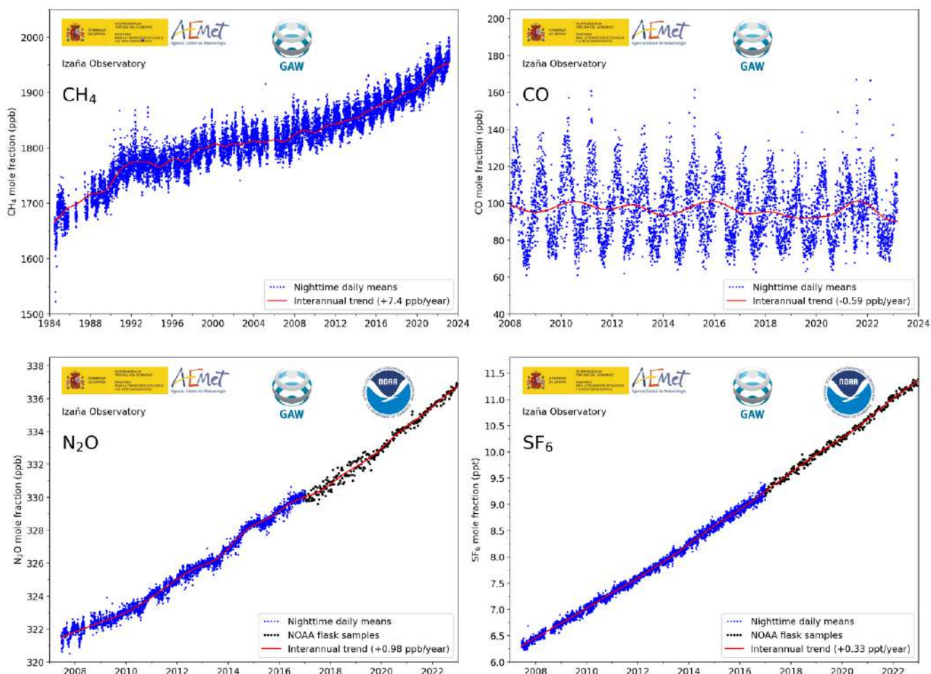
Figure 4.4. CH 4 , CO, N 2 O and SF 6 IZO time series. N 2 O and SF 6 measurements by IZO analysers from the year 2017 onwards are temporarily unavailable due to technical problems and system updates. Data from 2017 to 2022 in these figures come from the NOAA Cooperative Air Sampling Network and are shown as black points.
