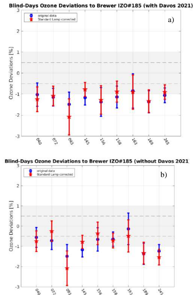
Figure 16.13. Initial period, percentage mean difference with the reference for the simultaneous direct sun measurements for all the participating instruments, with and without the standard lamp correction, in the stray-light free OSC region ( OSC < 900 ). a) Summary of the blind comparison considering the calibration obtained during the 2021 campaign. b) The same results when taking the configurations prior to the 2021 campaign for Brewers #040, #072, #156, #158, #163 and #254.
