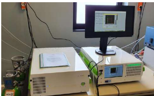
Figure 5.5. EcoPhysics CraNO x II analyser at the Izaña Observatory.
