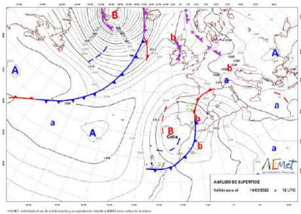
Figure 13.20. Surface pressure analysis and fronts, 14/03/2022 12 UTC.
