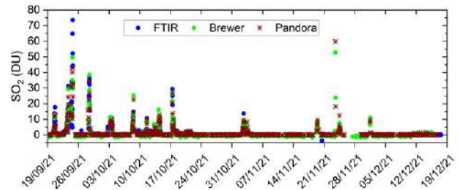
Figure 23.22. Total column SO 2 from Brewer, Pandora, and FTIR instruments in IZO (19/9/2021- 19/12/2021).
