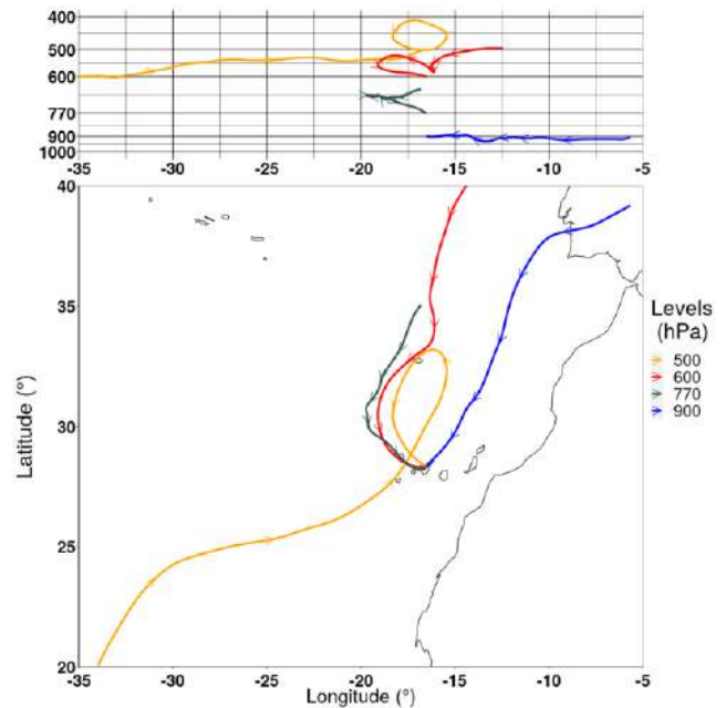
Figure 13.30. FLEXTRA back-trajectories corresponding to 24 September 2021 at 12:00 hours for arrival pressure levels of 900, 770, 600, and 500 hPa at the Izaña Observatory. Reprinted from García et al. (2023).
