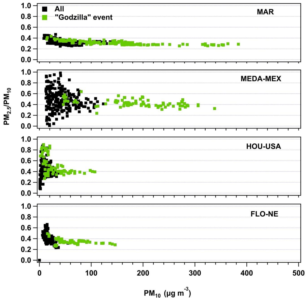
Figure 15. Ratio of fine ( PM_{2.5} ) to coarse ( PM_{10} ) particle mass as a function of PM_{10} during the peak of the Godzilla dust event (green squares, e.g., June 19-24 at MAR ) and for the whole period of study (black shading) between June 18 and July 2, observed at Martinique (MAR), Merida-Mexico (MEDA-MEX), Houston (HOU-USA), and Florida- Jacksonville (Florida-NE).
