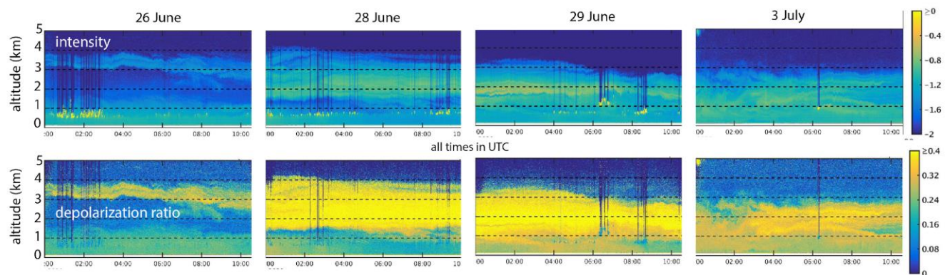
Figure 8. Evolution of the backscattered intensity record (upper panels) and the volume depolarization ratio (lower panels) above Miami, FL, from June 26 through July 3, 2020, as observed by a micropulse lidar. The logarithmic color scales should be interpreted qualitatively. The upper panels show increasing amounts of aerosol being advected over Miami with time. The lower panels show that the SAL subsides as the dust event moves through the region. The volume depolarization ratios are relatively large, which could be interpreted to mean that the aerosol is dominated by aspherical particles (e.g., mineral dust) that overwhelm other types of aerosols that are more spherical, most likely sea salt.
