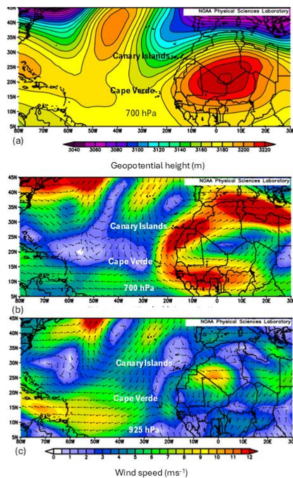
Figure 4. Time-averaged (a) Geopotential height at 700 hPa (m); (b) Vector wind at 700 hPa, (c) Vector wind at 925 hPa for the period June 1-13, 2020, in the geographical domain 5°N-45°N, 80°W-30°E, under negative NAFDI phase. (Source: NCEP/NCAR reanalysis)
