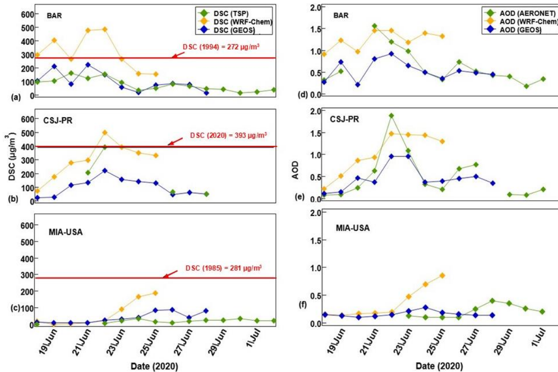
Figure 17. Dust mass surface concentrations measured (DSC, TSP, green) and modeled (DSC, WRF-CHEM, yellow; GEOS, blue) at BAR (a), CSJ-PR (b), and MIA-USA (c) during June 18 - July 2. The red horizontal lines represent the highest registered measured DSC at (a) BAR (272 \mu\text{g}/\text{m}^3 in April 1994), (b) CSJ-PR (393 \mu\text{g}/\text{m}^3 in June 2020), and (c) MIA-USA (281 \mu\text{g}/\text{m}^3 in November 1985). BAR and MIA-USA concentrations are based on the historical records (Zuidema et al. 2019). CSJ-PR is based on the US-EPA historical records in Puerto Rico and the CSJ-PR data. Dust model AOD outputs initiated on June 18 by WRF-Chem (yellow) and GEOS (blue) along with AOD from AERONET (green) for BAR (d), CSJ-PR (e), and MIA-USA (f) for June 18-28. DSC (a, b and c) and AOD (d, e and f) forecasts are seven days (3-hour resolution) for WRF-CHEM and ten days (1-hour resolution) for GEOS.
