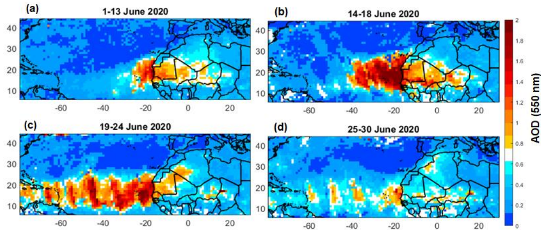
Figure 5. Time-averaged MODIS AOD at 550 nm in the geographical domain 5°N-45°N, 80°W-30°E for (a) June 1-13, 2020, (b) June 14-18, 2020, (c) June 19-24, 2020, and (d) June 25-30, 2020. (Source: MODIS AOD data used in this work can be freely obtained at https://giovanni.gsfc.nasa.gov/giovanni/ ).
