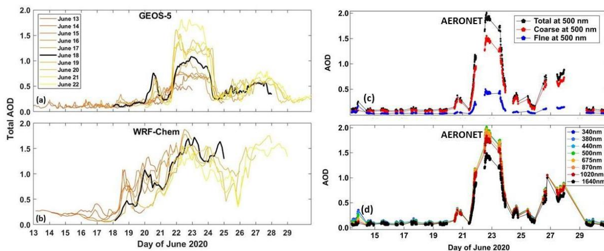
Figure 10. (a) GEOS forecast total AOD and (b) WRF-Chem forecast total AOD at CSJ-PR, color-coded by the forecast initialization time. The 00Z June 18 forecast is highlighted by the thick black line. (c) CSJ-PR AERONET total coarse and fine AOD, and (d) CSJ-PR AERONET daily mean AOD obtained in all 8 spectral channels (340, 380, 440, 500, 675, 870, 1020, and 1640 nm).
