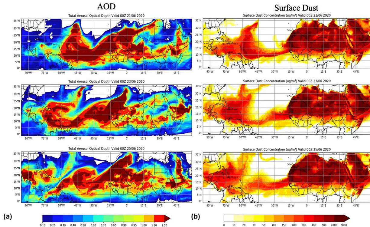
Figure 9. WRF-Chem prediction of aerosol optical depth (AOD) (a) and surface dust concentration (b) initialized June 20, 2020, 00Z and valid for June 21, 2020, 00Z (upper), June 23, 2020, 00Z (middle), and June 25, 2020, 00Z (lower), respectively.
