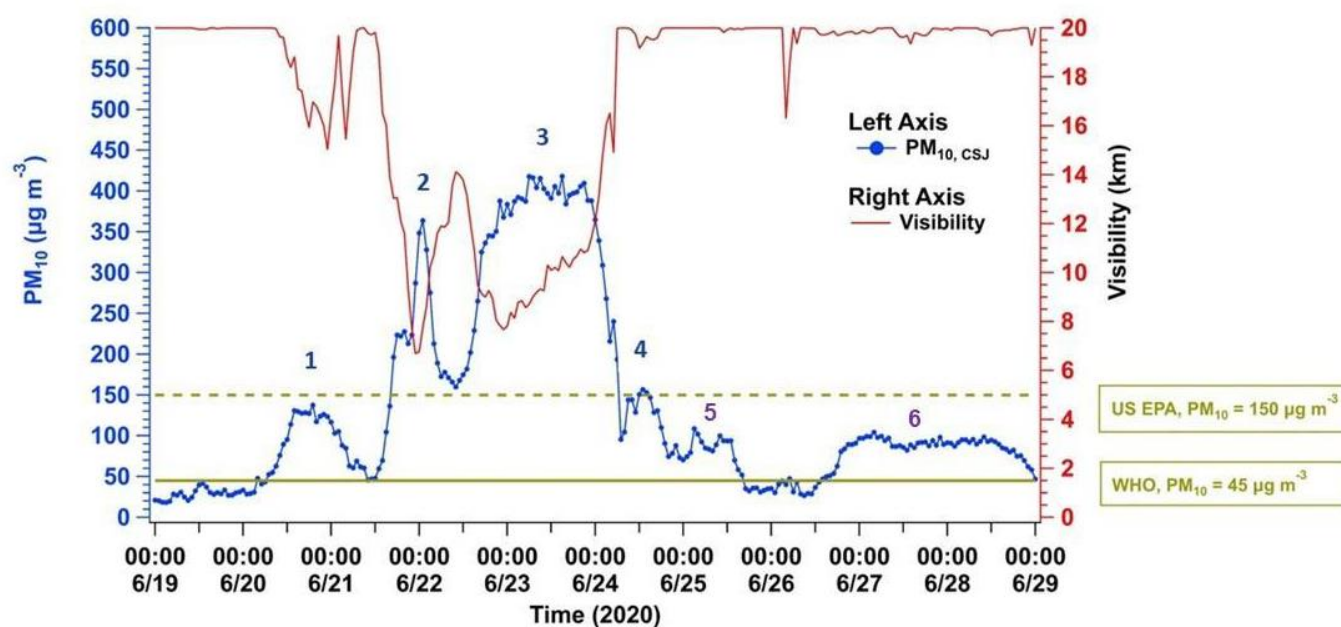
Figure 12. Puerto Rico (CSJ-PR) PM_{10} mass concentrations (primary y-axis) and visibility (secondary y-axis) from June 19 - 29. The first dust pulse (Godzilla) is represented by peaks 1 to 5. Peak 6 represents a 2nd dust pulse. The gold horizontal lines show the US EPA and WHO 24-h PM_{10} guidelines.
