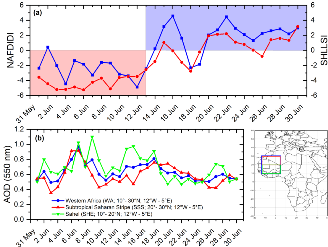
Figure 3. Time series of a) NAFDI daily index (NAFDIDI) and the Saharan Heat low Longitudinal Shift Index (SHLLSI), and b) daily MODIS Aerosol Optical Depth (AOD) at 550 nm for June 2020 over the African dust source regions.
