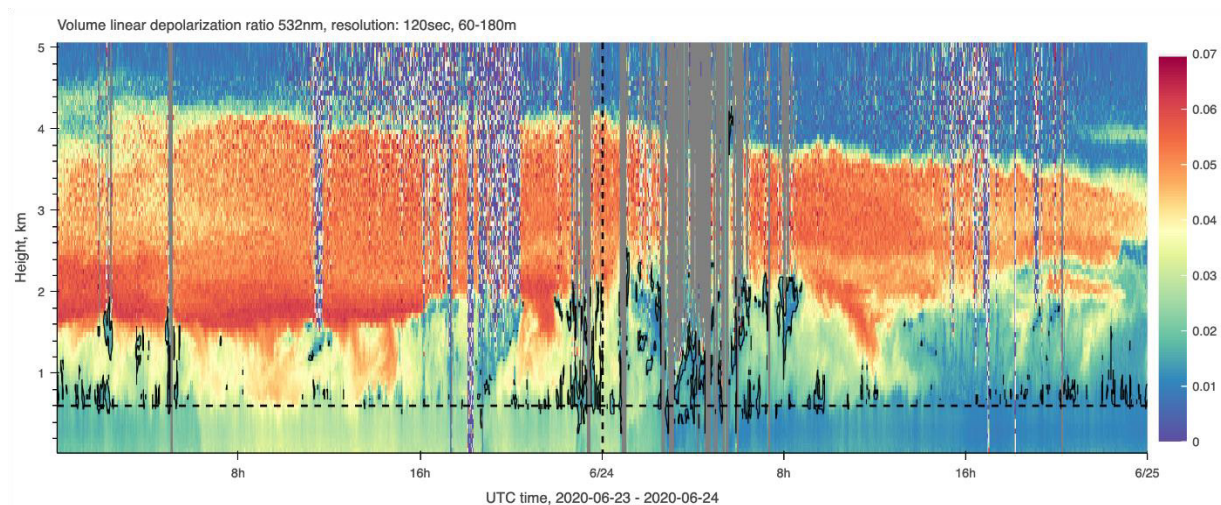
Figure 7. Evolution of the Godzilla dust plume above Barbados (13.163N; -59.429W) during June 23-24, 2020, based on measurements of volume depolarization ratio using the CORAL LIDAR. The days with the maximum aerosol loading measured with filters at Ragged Point are associated with a very high-volume depolarization ratio. Dust, having more aspherical aspect ratios, will produce higher values of the depolarization ratio, with all other properties remaining unchanged. Black contours indicate clouds. The dashed vertical line indicates 0:00 UTC on June 24. The dashed horizontal line indicates the approximate cloud base (estimated to be at 600 m). The plumes seen descending from the SAL base suggest that dust is actively transferred from the SAL to the marine boundary layer air by convective mixing processes.
