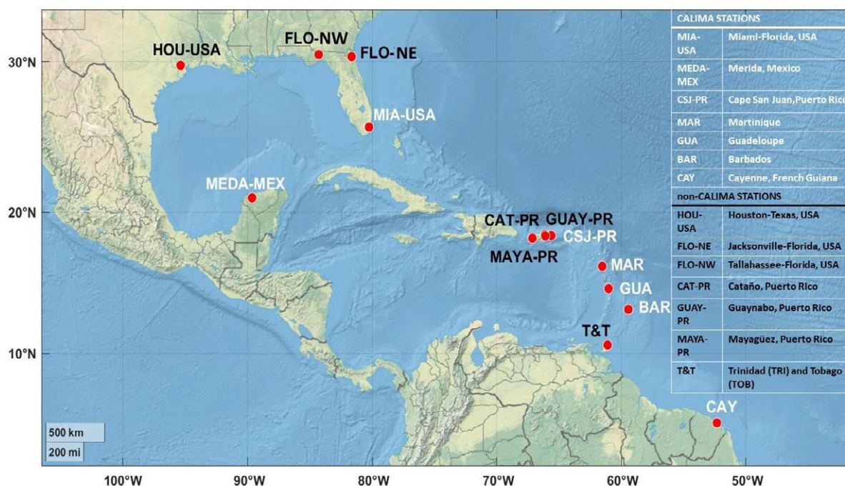
Figure 2. Map of the Greater Caribbean Basin, defined as encompassing the island nations and Caribbean coastal states, including the southeastern US, central and northern South America, showing the CALIMA 2020 sampling locations: Cayenne, Trinidad and Tobago, Ragged Point - Barbados, Martinique, Guadeloupe, Cape San Juan-Puerto Rico, Cataño-Puerto Rico, Mayagüez-Puerto Rico, Guaynabo-Puerto Rico, Merida-Mexico, Miami, Jacksonville, Tallahassee, and Houston. The names in black are contributing stations but non-CALIMA stations. The map is created using Natural Earth in MATLAB.
