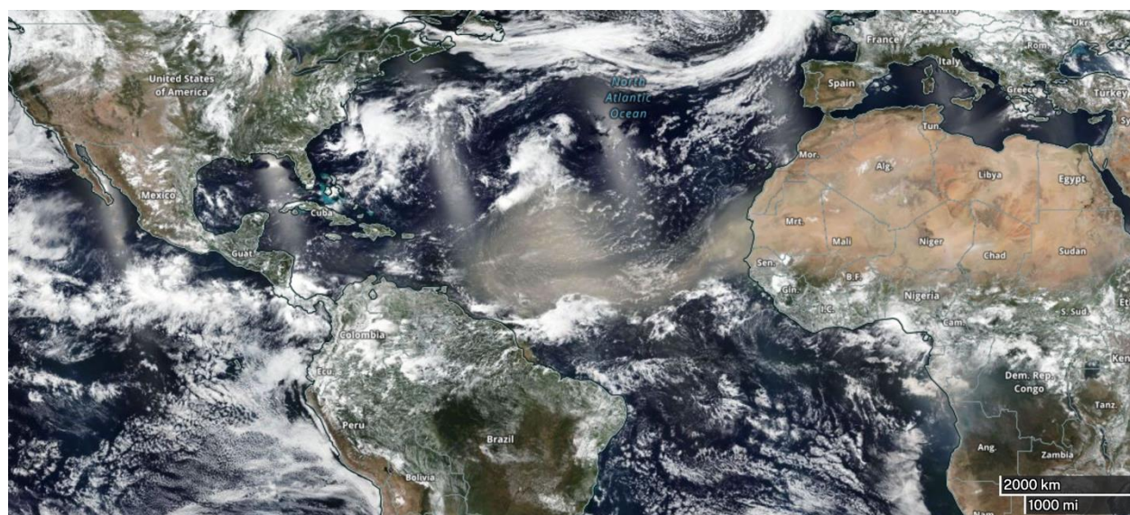
Figure 1. Dust plumes over the tropical Atlantic and the Greater Caribbean Basin on 20 June 2020 observed by the VIIRS sensor aboard the Suomi-NPP satellite, visualized with NASA WorldView. VIIRS is a polar-orbiting satellite. The coherent bright bars, located at a slight angle from the vertical, are due to the specular reflection of sunlight from the ocean surface; a bar is generated on each overpass.
