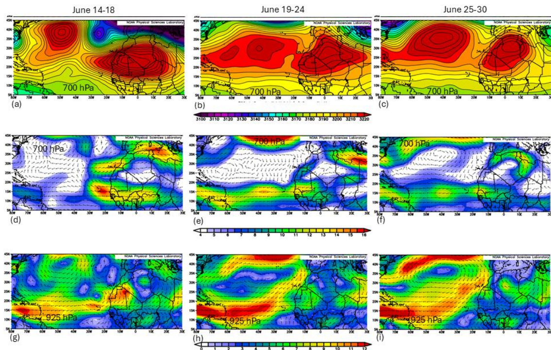
Figure 6. Time-averaged geopotential height at 700 hPa (m) for (a) June 14-18, (b) June 19-24, and (c) June 25-30; Time-averaged vector wind at 700 hPa ( \text{ms}^{-1} ) for (d) June 14-18, (e) June 19-24, and (f) June 25-30; Time-averaged vector wind at 925 hPa ( \text{ms}^{-1} ) for (g) June 14-18, (h) June 19-24, and (i) June 25-30, in the geographical domain 5^{\circ} N- 45^{\circ} N, 80^{\circ} W- 30^{\circ} E, under positive NAFDI phase. (Source: NCEP/NCAR reanalysis)
