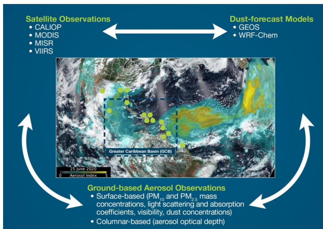
Figure 18. Progression and extent of the Godzilla dust event, ground-based CALIMA and non-CALIMA stations, ground-based and satellite observations, and dust forecast models. Source for the satellite image: OMPS aerosol index and the VIIRS visible image both from NASA/NOAA's Suomi NPP satellite on June 25.
