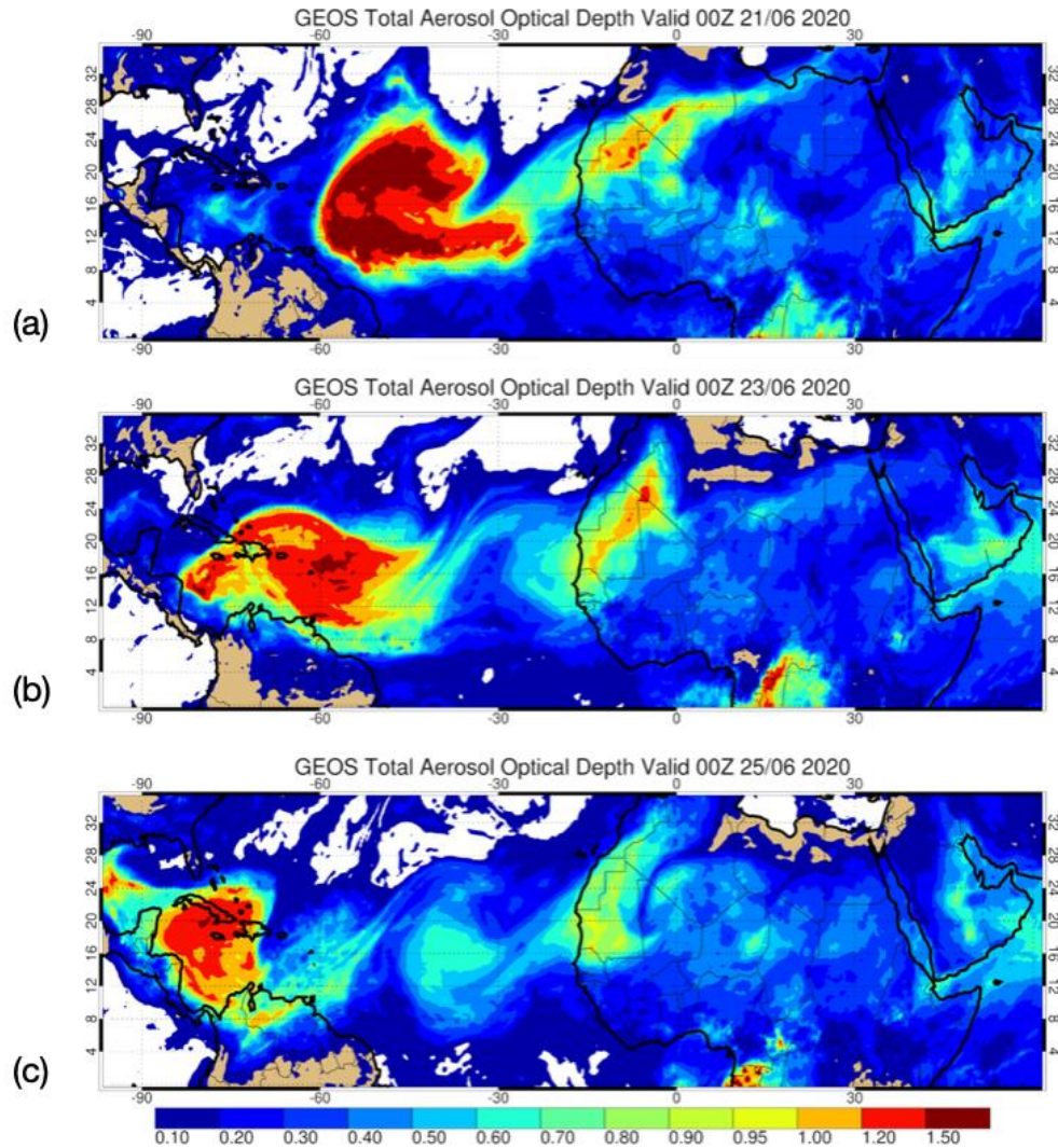
Figure 11. Forecast total AOD from the GEOS 0Z June 20, 2020, forecast for each of (a) 00Z June 21, 2020, (b) 00Z June 23, 2020, and (c) 00Z June 25, 2020.
