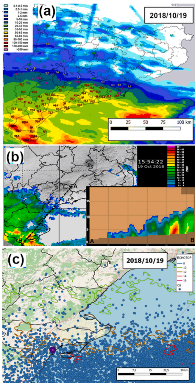
Fig. 14. 19 October 2018: (a) Daily rainfall field estimated from the combination of rain gauge and radar data, showing the locations of XEMA stations; (b) radar reflectivity (dBZ) from CAPPI-4 km at 15:54 UTC, including the vertical section between points A and B; (c) cloud-to-ground electrical discharges and maximum echotop-12 dBZ height (km). Data source: SMC.
