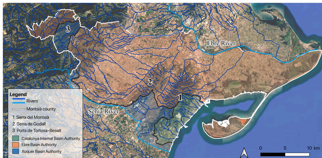
Fig. 2. Hydrographic and orographic map of Montsià county (white line), showing the Sènia River, the Ebre River, the Montsià range (Serra del Montsià) (1), the Godall range (Serra de Godall) (2), and the mountain range of Els Ports de Tortosa-Beseit (3). The sectors belonging to the different hydrographic basins are shown in different colors. Elaborated from Google maps.
