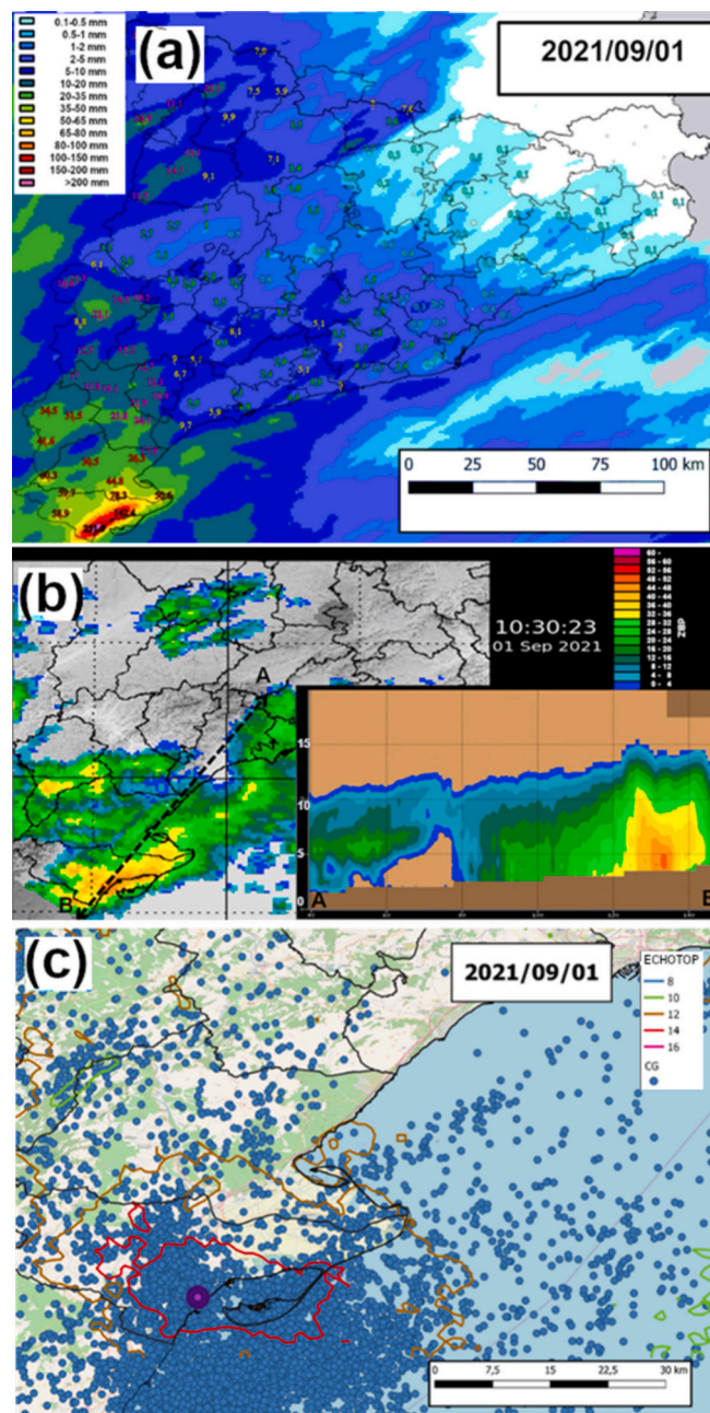
Fig. 15. 1 September 2021: (a) Daily rainfall field estimated from the combination of rain gauge and radar data, showing the locations of XEMA stations; (b) radar reflectivity (dBZ) from CAPPI-4 km at 10:30 UTC, including the vertical section between points A and B; (c) cloud-to-ground electrical discharges and maximum echotop-12 dBZ height (km). Data source: SMC.
