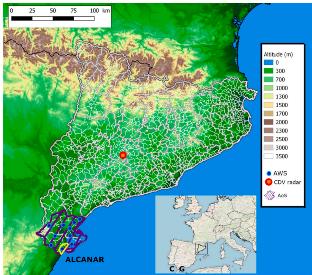
Fig. 1. Orographic map of Catalonia showing the locations of Baix Ebre and Montsià counties (Area of Study, AoS, shaded), XEMA network meteorological stations within these counties (blue circles, AWS), the SMC meteorological radar at La Panadella (red circle, CDV), and Alcanar municipality (yellow). The Strait of Gibraltar (G) and Cape San Vicente (C), referenced in the text, are also shown. (For interpretation of the references to colour in this figure legend, the reader is referred to the web version of this article.)
