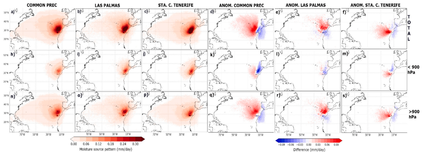
Fig. 8. Moisture source patterns (in mm/day) contributing to the Canary Islands from 1985 to 2022. Columns one to three show moisture sources, and four to six their anomalies with respect to the historical pattern, for days with precipitation in both provinces, only in Las Palmas, and only in Santa Cruz de Tenerife. Rows represent the fields for the entire atmospheric vertical column, the layer from the surface to 900 hPa, and the layer above 900 hPa.
