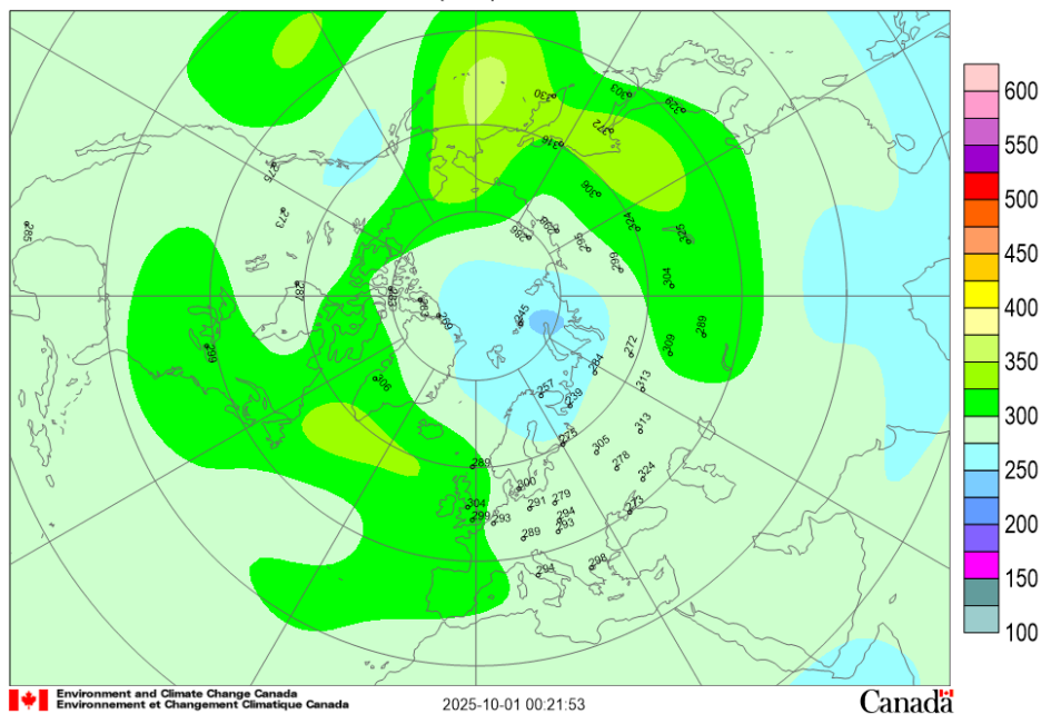
Mean total ozone (DU), 2025/09/01-2025/09/30
