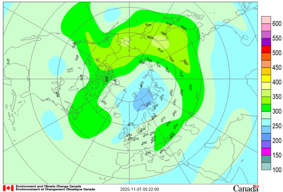
Mean total ozone (DU), 2025/10/01-2025/10/31
