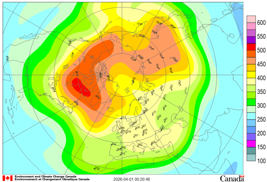
Mean total ozone (DU), 2026/03/01-2026/03/31
