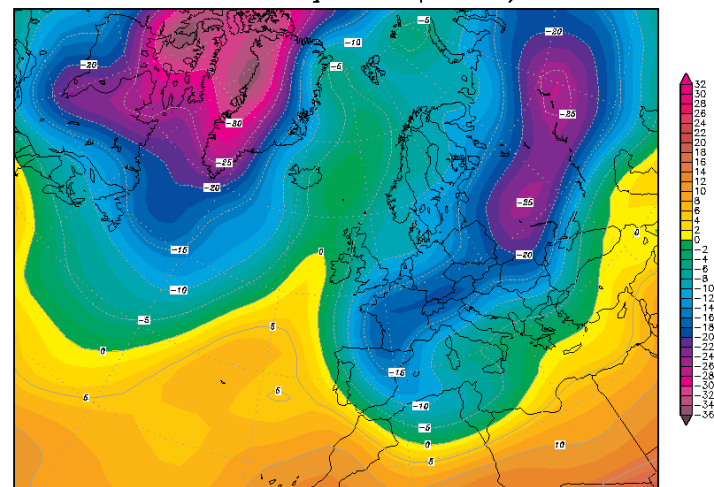
03FEB1956 00Z 850 hPa Temperatur (Grad C)
