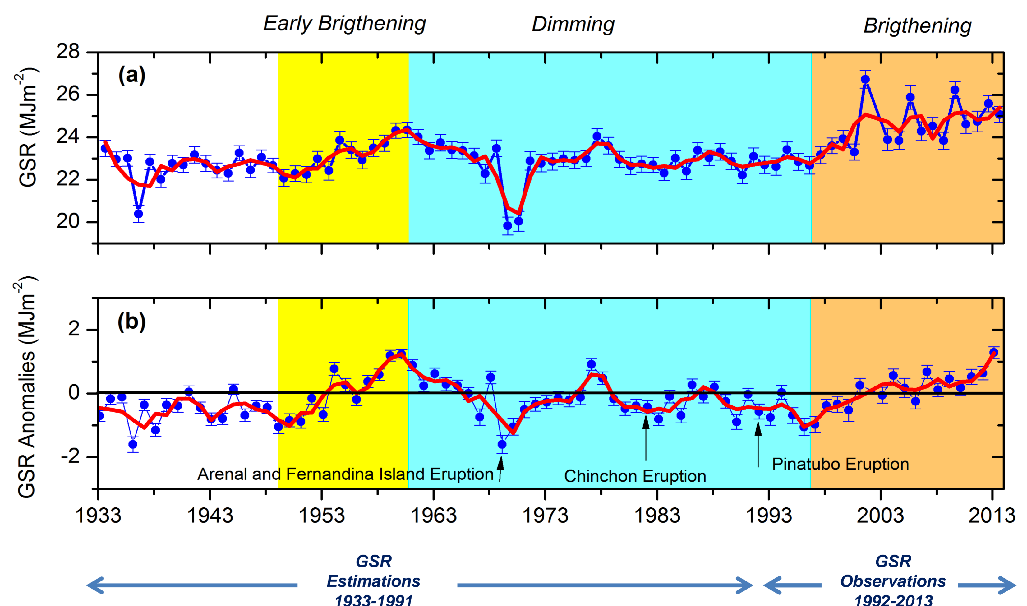
Figure 4.- Time series of the annual means of the (a) GSR and (b) GSR anomalies from 1933 to 2013 at IZA. The error bars indicate \pm 1 SEM (standard error of the mean). The arrows indicate the eruptions of Arenal and Fernandina (1968), Chinchón (1982) and Pinatubo (1991). Five-yr moving average is shown in red. (Time series has been deseasonalised by subtracting the averaged GSR annual cycle, obtaining the annual mean anomalies time series).
