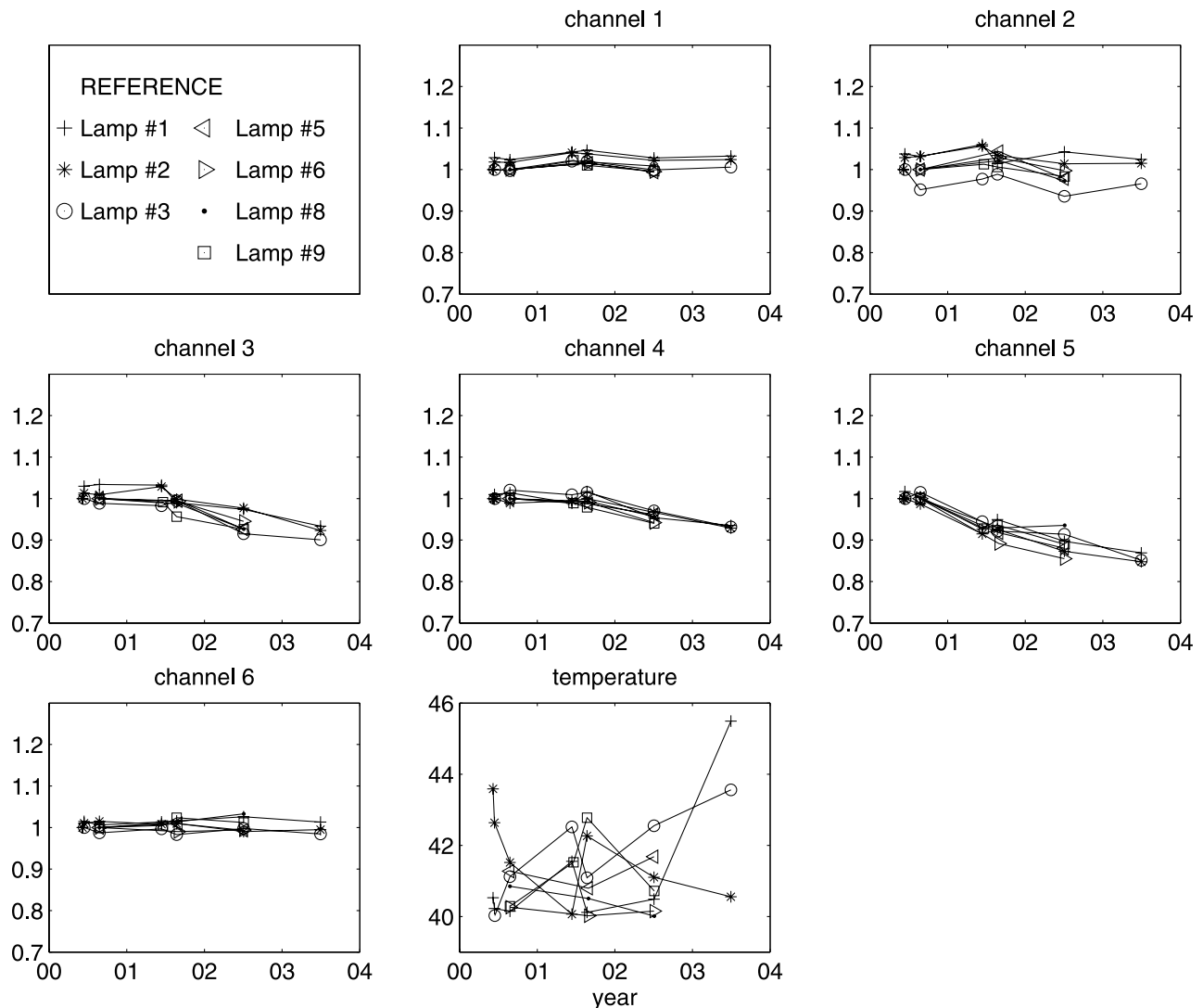
Figure 3. The lamp test time series of the reference NILU-UV measured at FMI during 2000–2003. See color version of this figure in the HTML.
