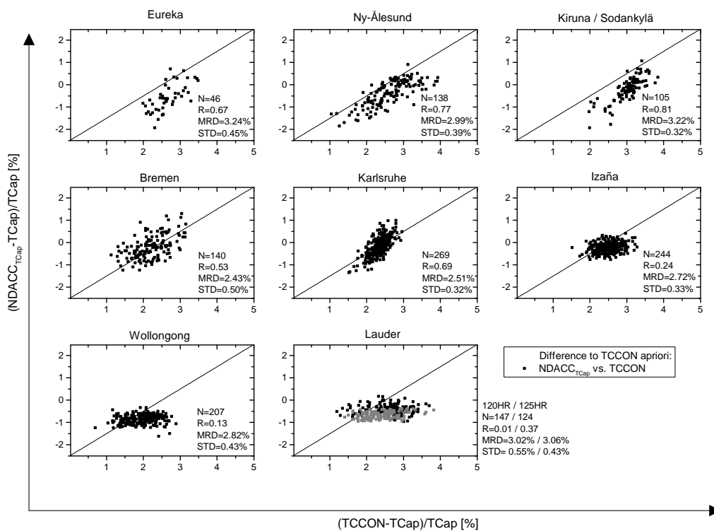
Figure B1. Correlation between (NDACC TCap -TCap) and (TCCON-TCap). The black line represents the one-to-one correlation shifted by 2.5%. The grey squares in the Lauder graph represent the data measured with the 125HR instrument, whereas the black squares are the data measured with the 120HR instrument.
